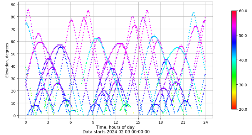
Time-elevation plot for station EIVI. Signal to Noise S1C Data file EIVI00ESP_R_2024040.xtr
