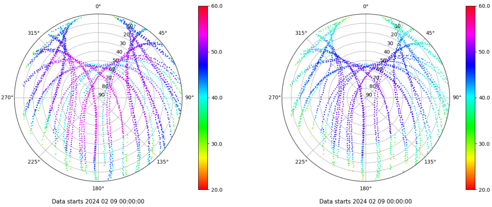
Skyplot for station EIVI. Signal to Noise S1C Data file EIVI00ESP_R_2024040.xtr Skyplot for station EIVI. Signal to Noise S2P Data file EIVI00ESP_R_2024040.xtr
