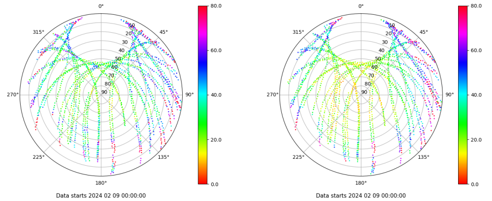
Skyplot for station EIVI. Parameter M1C Data file EIVI00ESP_R_2024040.xtr Skyplot for station EIVI. Parameter M2P Data file EIVI00ESP_R_2024040.xtr
