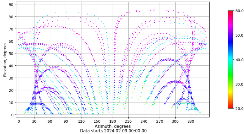
Azimuth-elevation plot for station EIVI. Signal to Noise S1C Data file EIVI00ESP_R_2024040.xtr
