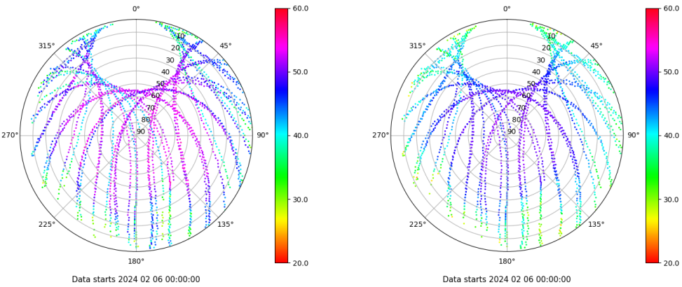
Skyplot for station EIVI. Signal to Noise S1C Data file EIVI00ESP_R_2024037.xtr Skyplot for station EIVI. Signal to Noise S2P Data file EIVI00ESP_R_2024037.xtr
