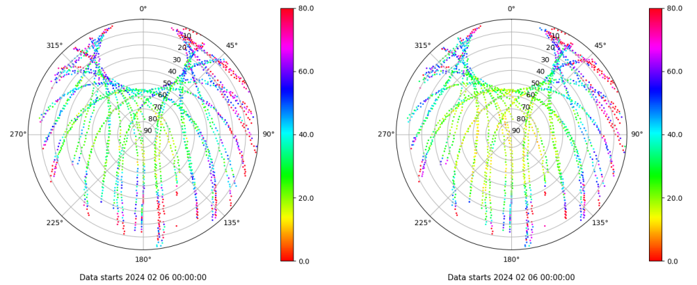
Skyplot for station EIVI. Parameter M1C Data file EIVI00ESP_R_2024037.xtr Skyplot for station EIVI. Parameter M2P Data file EIVI00ESP_R_2024037.xtr
