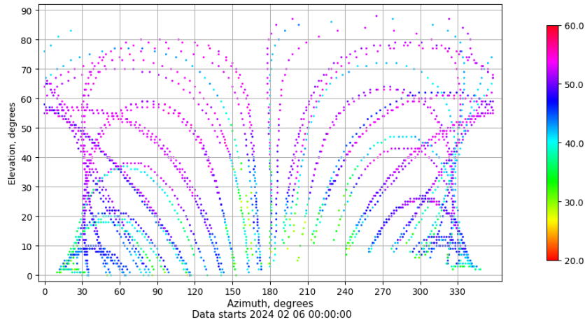
Azimuth-elevation plot for station EIVI. Signal to Noise S1C Data file EIVI00ESP_R_2024037.xtr
