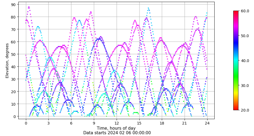
Time-elevation plot for station EIVI. Signal to Noise S1C Data file EIVI00ESP_R_2024037.xtr
