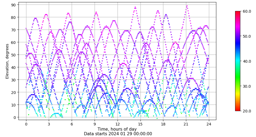
Time-elevation plot for station EIVI. Signal to Noise S1C Data file EIVI00ESP_R_2024029.xtr
