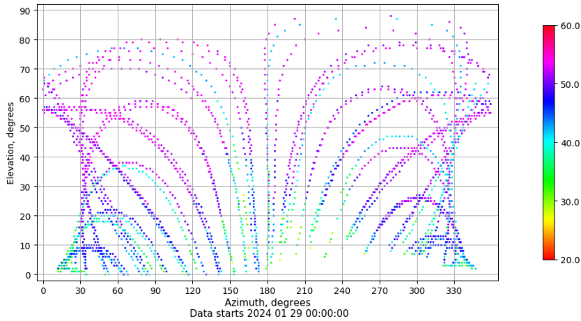
Azimuth-elevation plot for station EIVI. Signal to Noise S1C Data file EIVI00ESP_R_2024029.xtr
