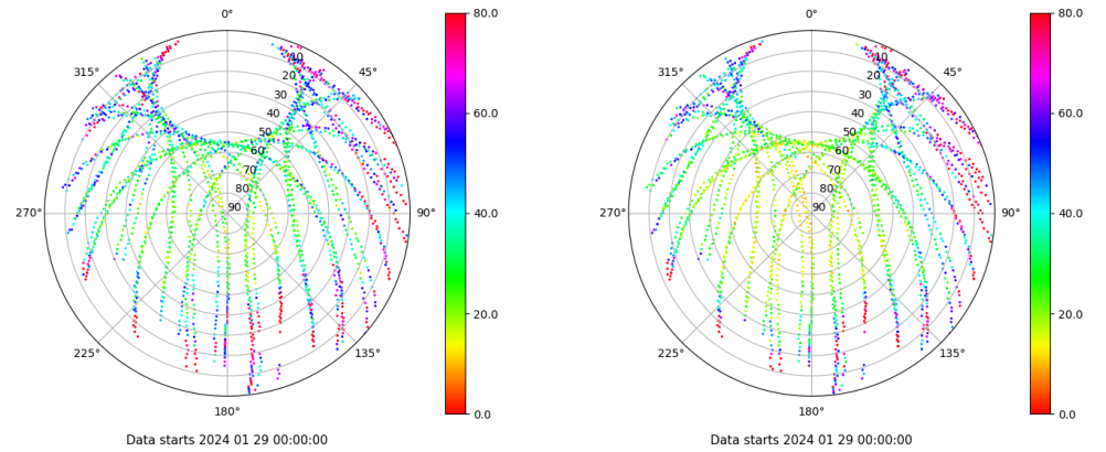
Skyplot for station EIVI. Parameter M1C Data file EIVI00ESP_R_2024029.xtr Skyplot for station EIVI. Parameter M2P Data file EIVI00ESP_R_2024029.xtr
