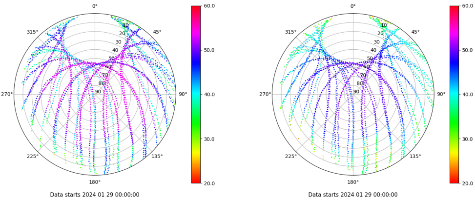
Skyplot for station EIVI. Signal to Noise S1C Data file EIVI00ESP_R_2024029.xtr Skyplot for station EIVI. Signal to Noise S2P Data file EIVI00ESP_R_2024029.xtr
