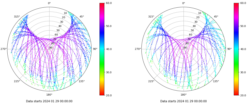
Skyplot for station EIVI. Signal to Noise S1C Data file EIVI00ESP_R_2024029.xtr Skyplot for station EIVI. Signal to Noise S2S Data file EIVI00ESP_R_2024029.xtr
