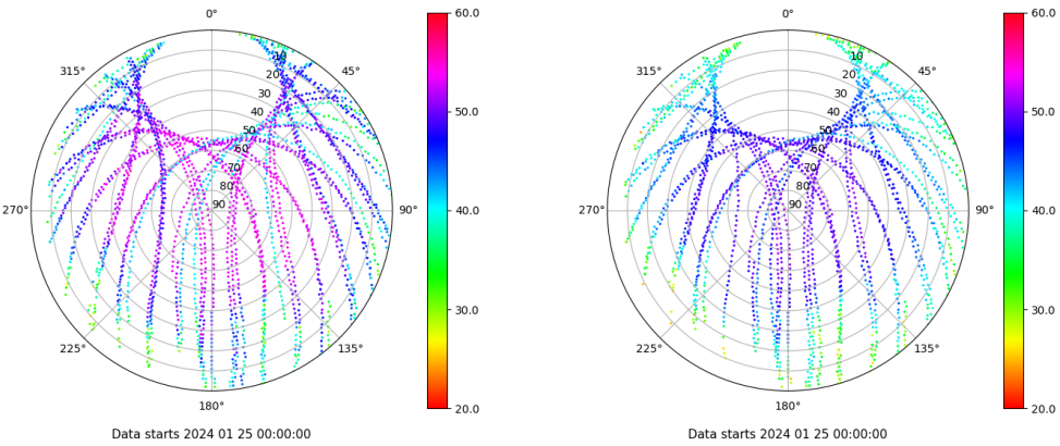
Skyplot for station EIVI. Signal to Noise S1C Data file EIVI00ESP_R_2024025.xtr Skyplot for station EIVI. Signal to Noise S2P Data file EIVI00ESP_R_2024025.xtr
