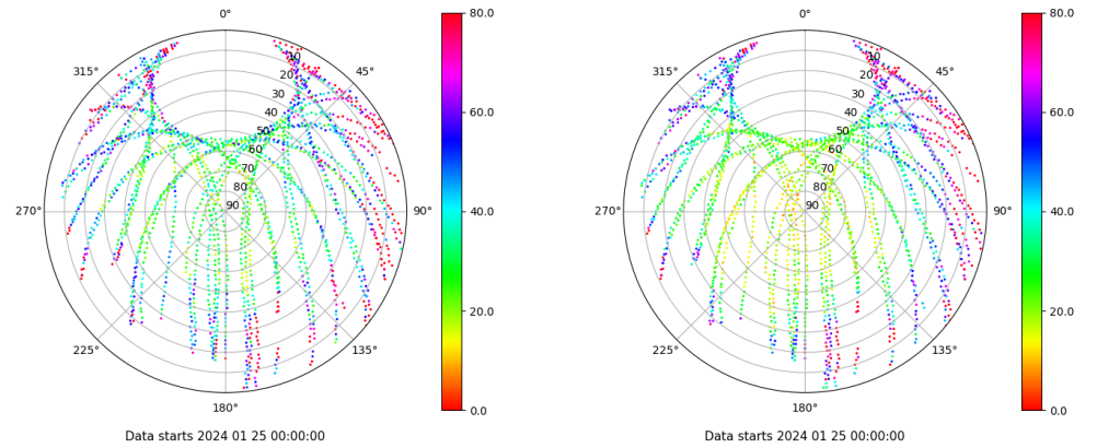
Skyplot for station EIVI. Parameter M1C Data file EIVI00ESP_R_2024025.xtr Skyplot for station EIVI. Parameter M2P Data file EIVI00ESP_R_2024025.xtr
