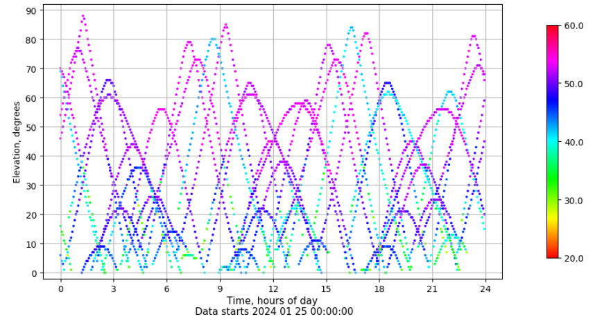
Time-elevation plot for station EIVI. Signal to Noise S1C Data file EIVI00ESP_R_2024025.xtr
