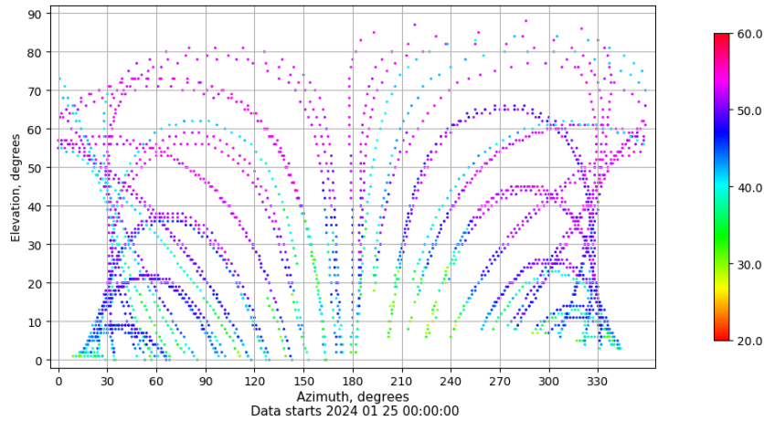
Azimuth-elevation plot for station EIVI. Signal to Noise S1C Data file EIVI00ESP_R_2024025.xtr
