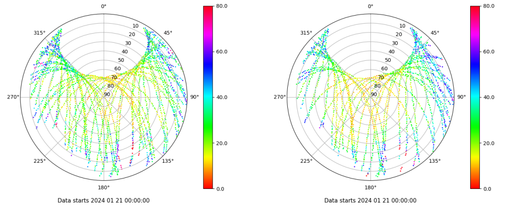
Skyplot for station EIVI. Parameter M1C Data file EIVI00ESP_R_2024021.xtr Skyplot for station EIVI. Parameter M2S Data file EIVI00ESP_R_2024021.xtr
