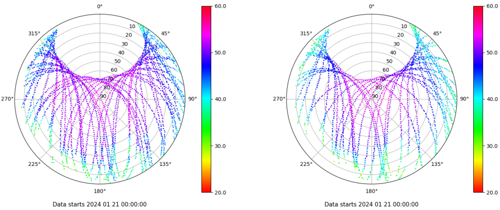
Skyplot for station EIVI. Signal to Noise S1C Data file EIVI00ESP_R_2024021.xtr Skyplot for station EIVI. Signal to Noise S2S Data file EIVI00ESP_R_2024021.xtr
