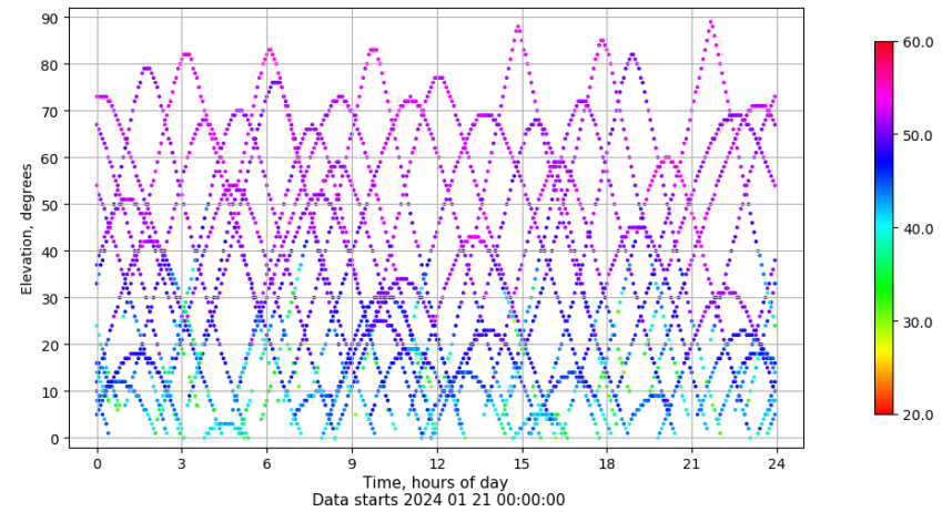
Time-elevation plot for station EIVI. Signal to Noise S1C Data file EIVI00ESP_R_2024021.xtr
