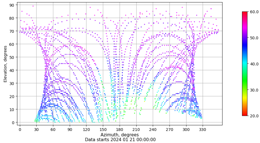
Azimuth-elevation plot for station EIVI. Signal to Noise S1C Data file EIVI00ESP_R_2024021.xtr
