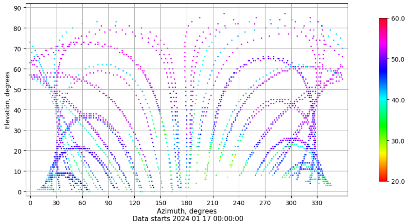
Azimuth-elevation plot for station EIVI. Signal to Noise S1C Data file EIVI00ESP_R_2024017.xtr
