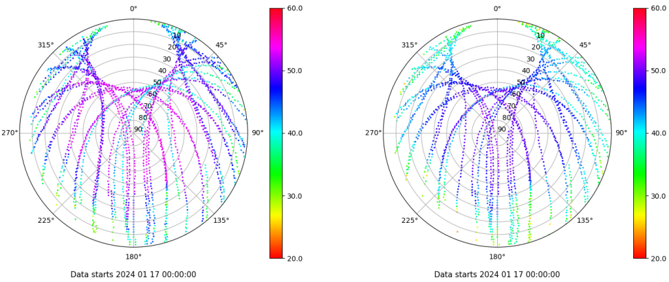
Skyplot for station EIVI. Signal to Noise S1C Data file EIVI00ESP_R_2024017.xtr Skyplot for station EIVI. Signal to Noise S2P Data file EIVI00ESP_R_2024017.xtr
