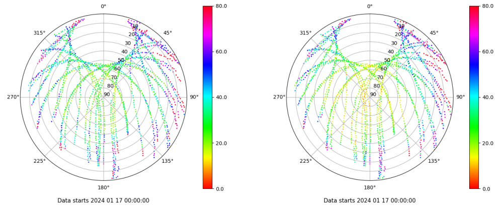
Skyplot for station EIVI. Parameter M1C Data file EIVI00ESP_R_2024017.xtr Skyplot for station EIVI. Parameter M2P Data file EIVI00ESP_R_2024017.xtr
