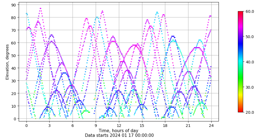
Time-elevation plot for station EIVI. Signal to Noise S1C Data file EIVI00ESP_R_2024017.xtr
