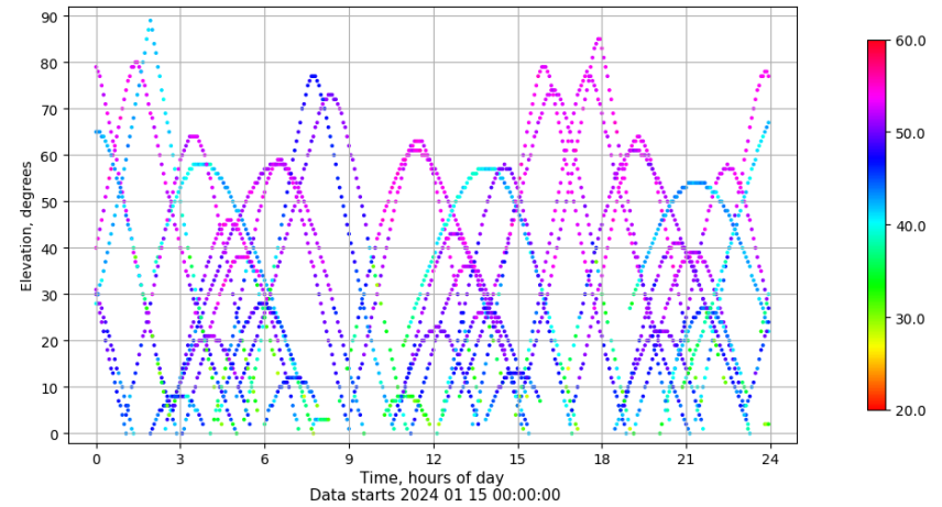
Time-elevation plot for station EIVI. Signal to Noise S1C Data file EIVI00ESP_R_2024015.xtr
