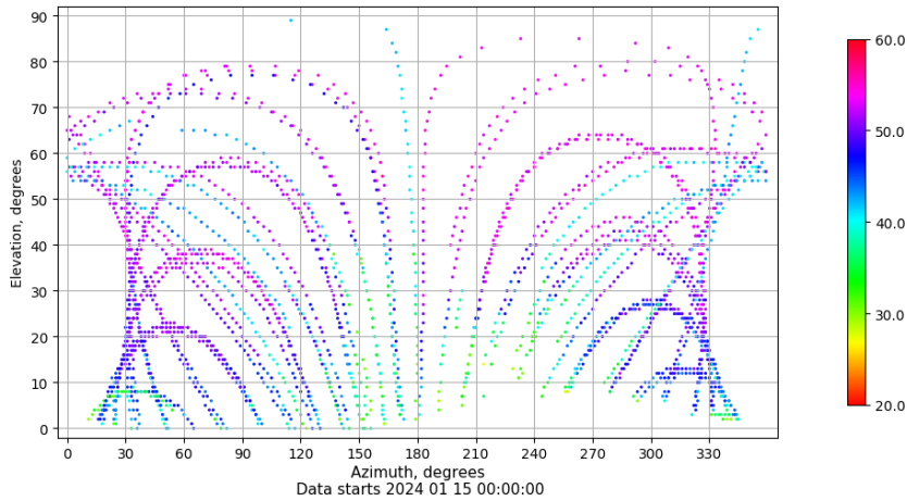
Azimuth-elevation plot for station EIVI. Signal to Noise S1C Data file EIVI00ESP_R_2024015.xtr
