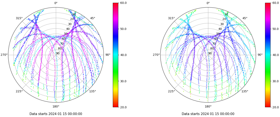
Skyplot for station EIVI. Signal to Noise S1C Data file EIVI00ESP_R_2024015.xtr Skyplot for station EIVI. Signal to Noise S2P Data file EIVI00ESP_R_2024015.xtr
