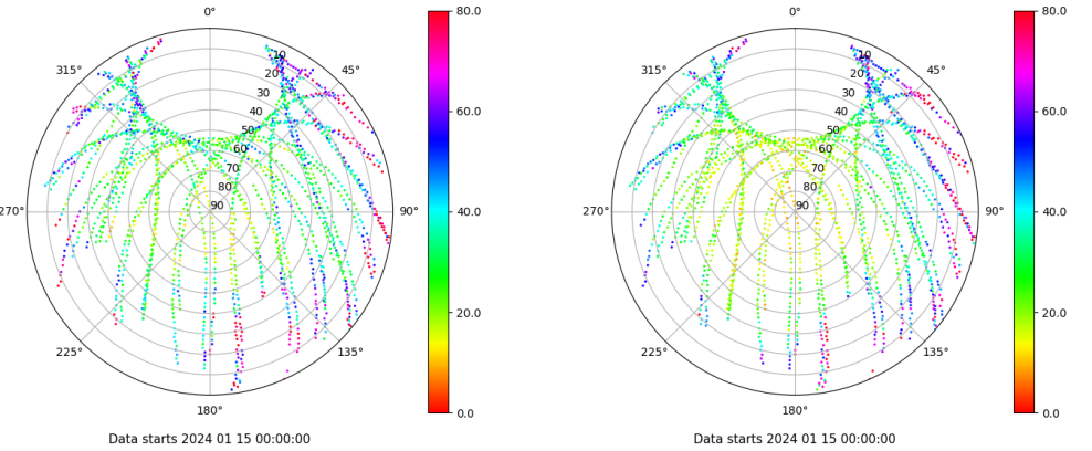
Skyplot for station EIVI. Parameter M1C Data file EIVI00ESP_R_2024015.xtr Skyplot for station EIVI. Parameter M2P Data file EIVI00ESP_R_2024015.xtr
