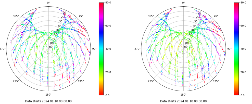
Skyplot for station EIVI. Parameter M1C Data file EIVI00ESP_R_2024010.xtr Skyplot for station EIVI. Parameter M2P Data file EIVI00ESP_R_2024010.xtr
