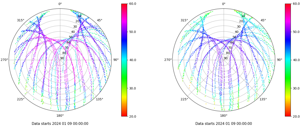
Skyplot for station EIVI. Signal to Noise S1C Data file EIVI00ESP_R_2024009.xtr Skyplot for station EIVI. Signal to Noise S2P Data file EIVI00ESP_R_2024009.xtr
