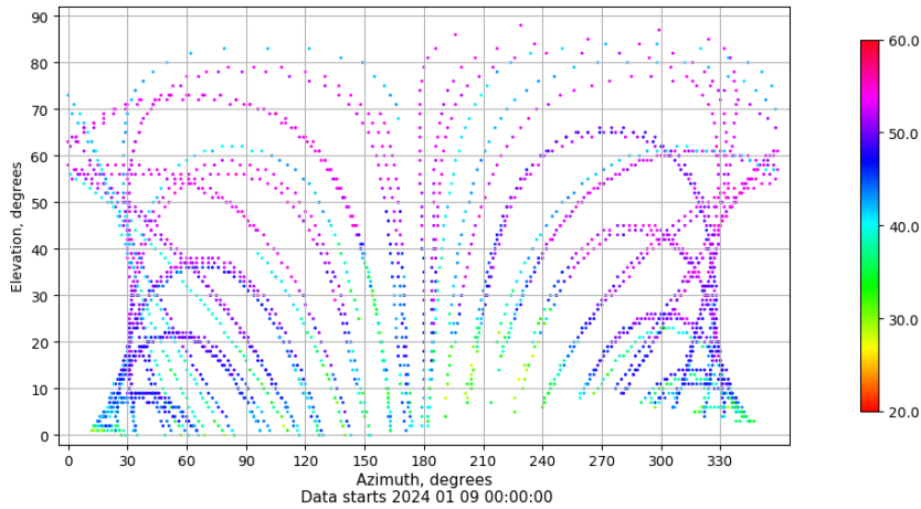
Azimuth-elevation plot for station EIVI. Signal to Noise S1C Data file EIVI00ESP_R_2024009.xtr
