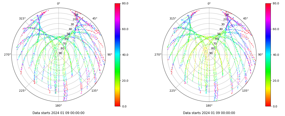
Skyplot for station EIVI. Parameter M1C Data file EIVI00ESP_R_2024009.xtr Skyplot for station EIVI. Parameter M2P Data file EIVI00ESP_R_2024009.xtr
