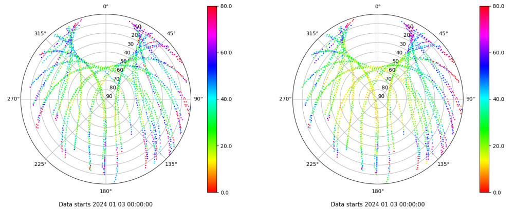
Skyplot for station EIVI. Parameter M1C Data file EIVI00ESP_R_2024003.xtr Skyplot for station EIVI. Parameter M2P Data file EIVI00ESP_R_2024003.xtr
