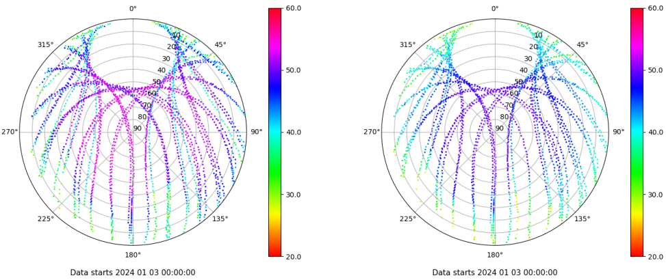
Skyplot for station EIVI. Signal to Noise S1C Data file EIVI00ESP_R_2024003.xtr Skyplot for station EIVI. Signal to Noise S2P Data file EIVI00ESP_R_2024003.xtr
