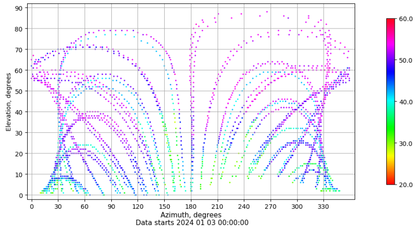
Azimuth-elevation plot for station EIVI. Signal to Noise S1C Data file EIVI00ESP_R_2024003.xtr
