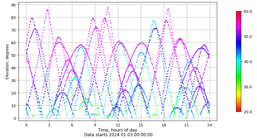
Time-elevation plot for station EIVI. Signal to Noise S1C Data file EIVI00ESP_R_2024003.xtr
