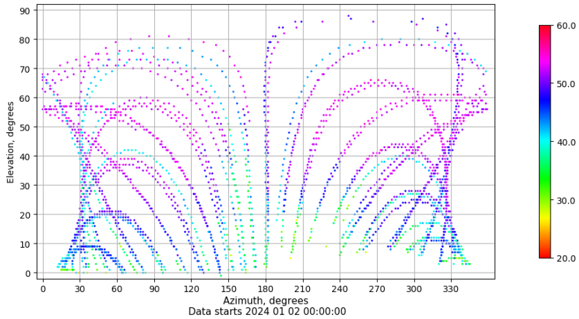
Azimuth-elevation plot for station EIVI. Signal to Noise S1C Data file EIVI00ESP_R_2024002.xtr
