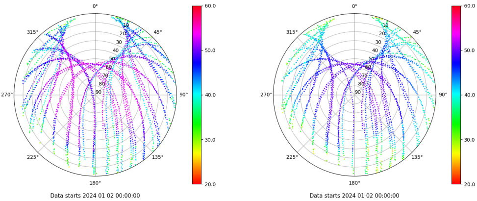
Skyplot for station EIVI. Signal to Noise S1C Data file EIVI00ESP_R_2024002.xtr Skyplot for station EIVI. Signal to Noise S2P Data file EIVI00ESP_R_2024002.xtr
