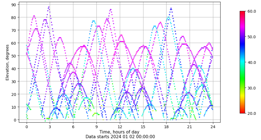
Time-elevation plot for station EIVI. Signal to Noise S1C Data file EIVI00ESP_R_2024002.xtr
