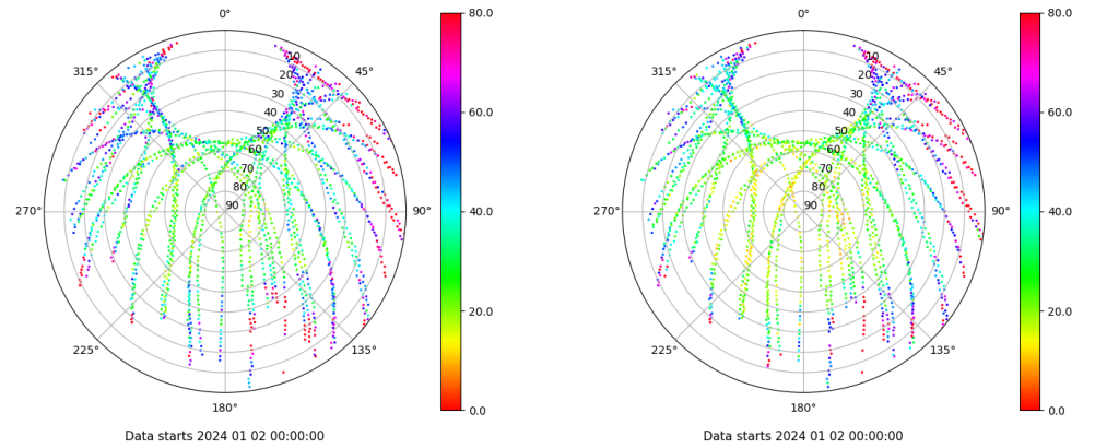
Skyplot for station EIVI. Parameter M1C Data file EIVI00ESP_R_2024002.xtr Skyplot for station EIVI. Parameter M2P Data file EIVI00ESP_R_2024002.xtr
