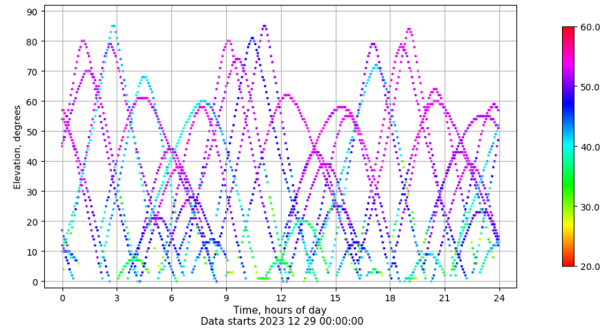
Time-elevation plot for station EIVI. Signal to Noise S1C Data file EIVI00ESP_R_2023363.xtr
