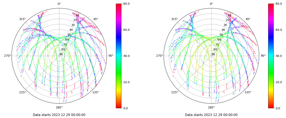
Skyplot for station EIVI. Parameter M1C Data file EIVI00ESP_R_2023363.xtr Skyplot for station EIVI. Parameter M2P Data file EIVI00ESP_R_2023363.xtr
