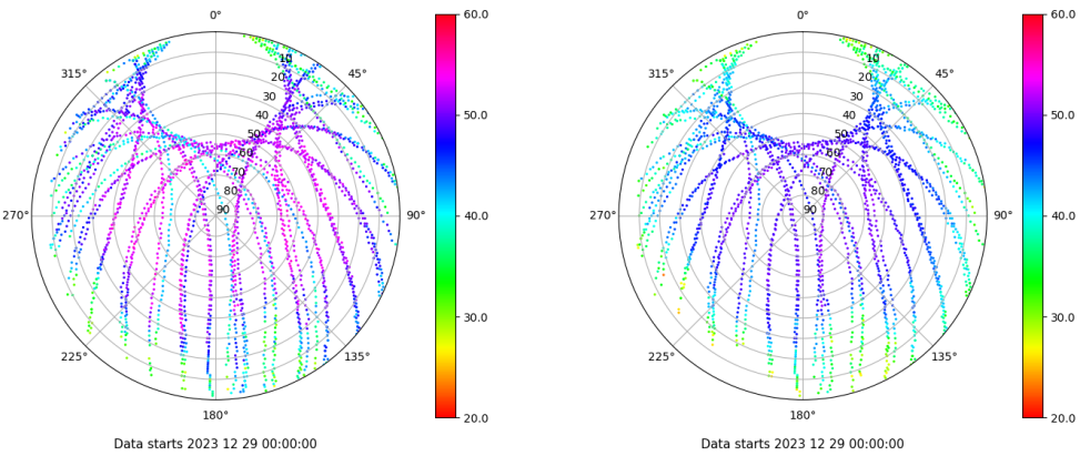
Skyplot for station EIVI. Signal to Noise S1C Data file EIVI00ESP_R_2023363.xtr Skyplot for station EIVI. Signal to Noise S2P Data file EIVI00ESP_R_2023363.xtr
