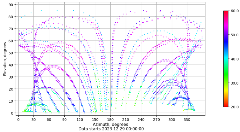
Azimuth-elevation plot for station EIVI. Signal to Noise S1C Data file EIVI00ESP_R_2023363.xtr
