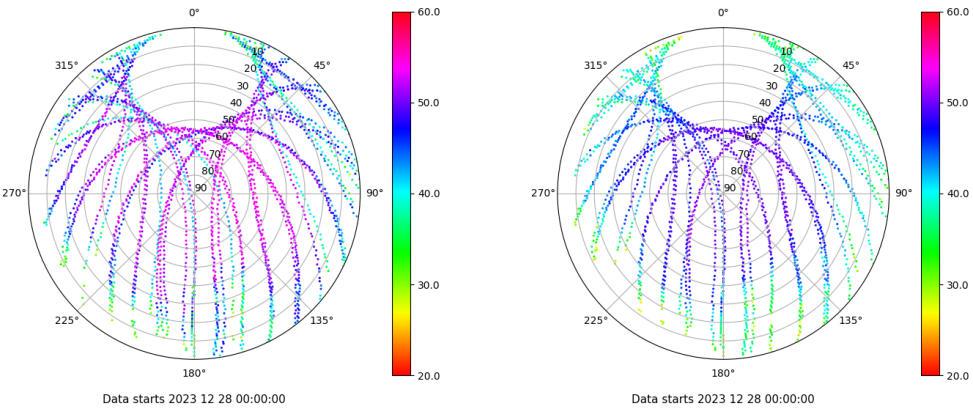
Skyplot for station EIVI. Signal to Noise S1C Data file EIVI00ESP_R_2023362.xtr Skyplot for station EIVI. Signal to Noise S2P Data file EIVI00ESP_R_2023362.xtr
