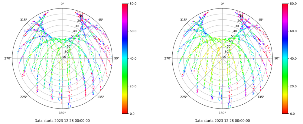
Skyplot for station EIVI. Parameter M1C Data file EIVI00ESP_R_2023362.xtr Skyplot for station EIVI. Parameter M2P Data file EIVI00ESP_R_2023362.xtr
