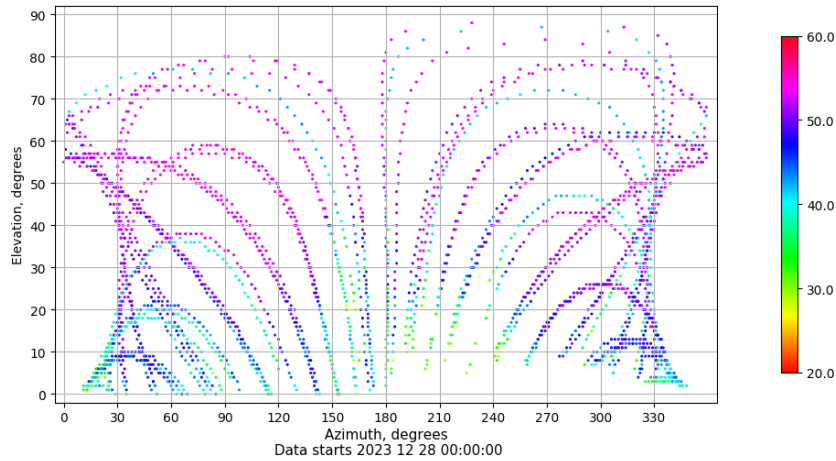
Azimuth-elevation plot for station EIVI. Signal to Noise S1C Data file EIVI00ESP_R_2023362.xtr
