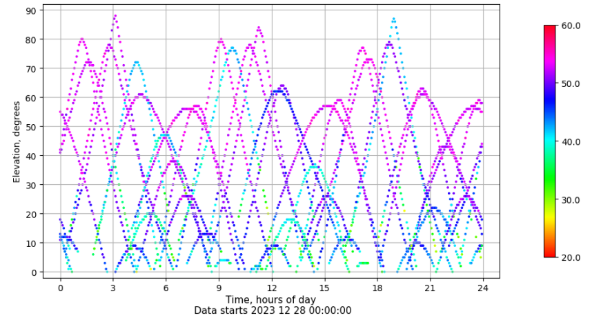
Time-elevation plot for station EIVI. Signal to Noise S1C Data file EIVI00ESP_R_2023362.xtr
