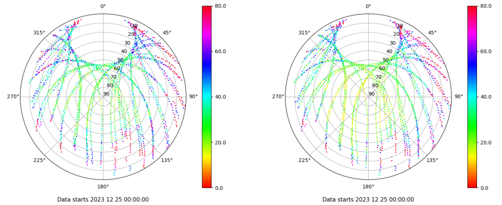
Skyplot for station EIVI. Parameter M1C Data file EIVI00ESP_R_2023359.xtr Skyplot for station EIVI. Parameter M2P Data file EIVI00ESP_R_2023359.xtr
