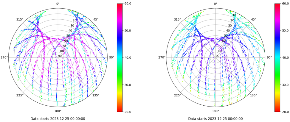
Skyplot for station EIVI. Signal to Noise S1C Data file EIVI00ESP_R_2023359.xtr Skyplot for station EIVI. Signal to Noise S2P Data file EIVI00ESP_R_2023359.xtr
