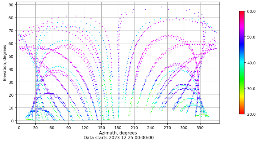
Azimuth-elevation plot for station EIVI. Signal to Noise S1C Data file EIVI00ESP_R_2023359.xtr
