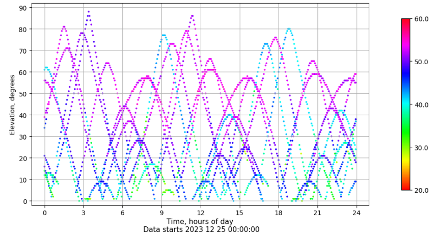
Time-elevation plot for station EIVI. Signal to Noise S1C Data file EIVI00ESP_R_2023359.xtr
