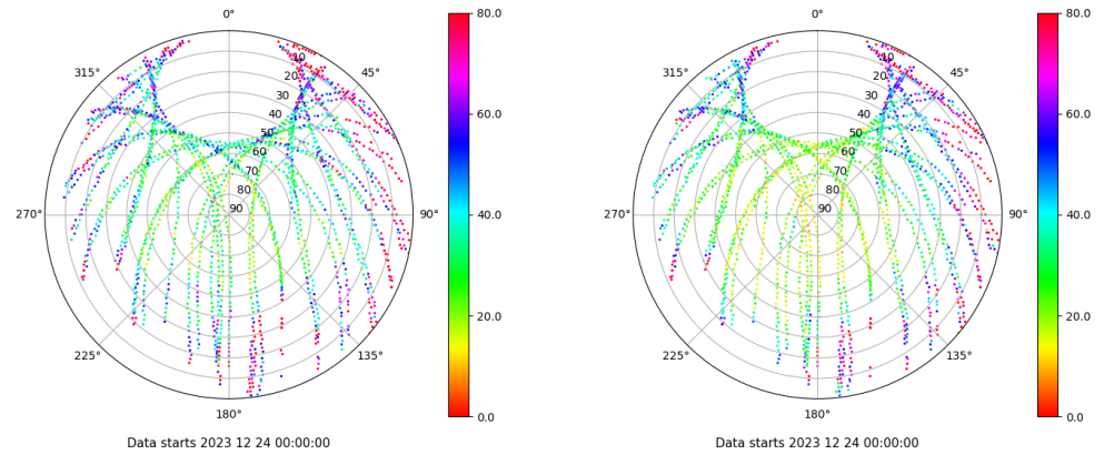
Skyplot for station EIVI. Parameter M1C Data file EIVI00ESP_R_2023358.xtr Skyplot for station EIVI. Parameter M2P Data file EIVI00ESP_R_2023358.xtr
