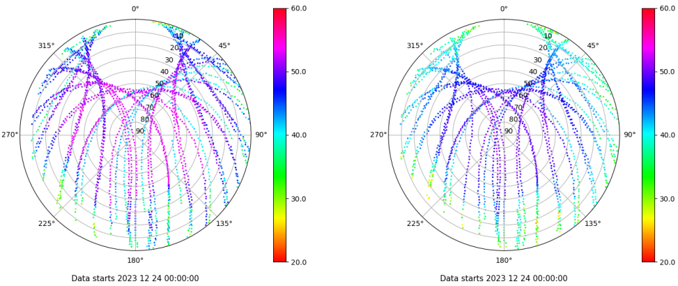
Skyplot for station EIVI. Signal to Noise S1C Data file EIVI00ESP_R_2023358.xtr Skyplot for station EIVI. Signal to Noise S2P Data file EIVI00ESP_R_2023358.xtr
