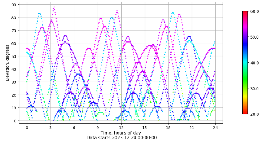
Time-elevation plot for station EIVI. Signal to Noise S1C Data file EIVI00ESP_R_2023358.xtr
