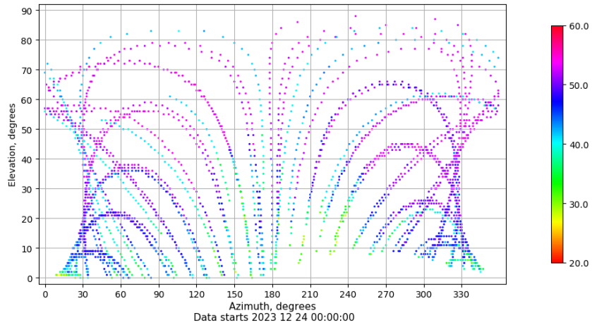
Azimuth-elevation plot for station EIVI. Signal to Noise S1C Data file EIVI00ESP_R_2023358.xtr
