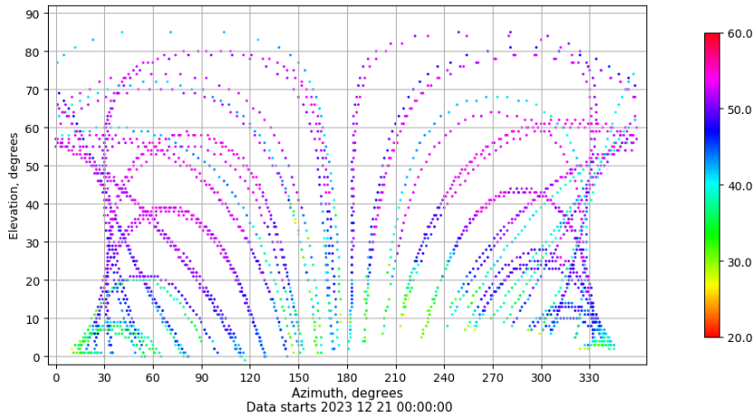
Azimuth-elevation plot for station EIVI. Signal to Noise S1C Data file EIVI00ESP_R_2023355.xtr
