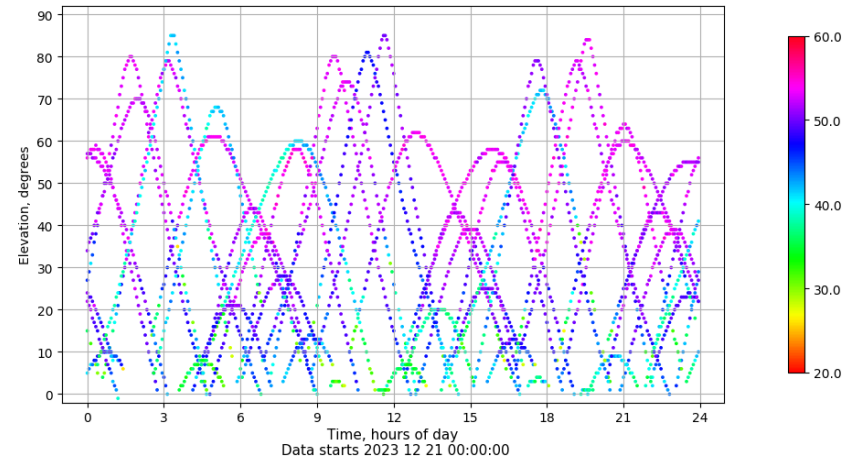
Time-elevation plot for station EIVI. Signal to Noise S1C Data file EIVI00ESP_R_2023355.xtr
