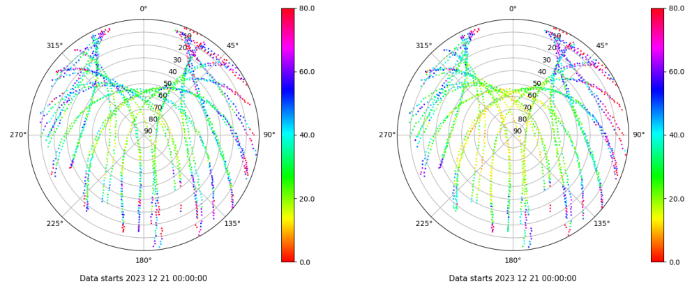
Skyplot for station EIVI. Parameter M1C Data file EIVI00ESP_R_2023355.xtr Skyplot for station EIVI. Parameter M2P Data file EIVI00ESP_R_2023355.xtr
