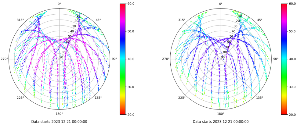
Skyplot for station EIVI. Signal to Noise S1C Data file EIVI00ESP_R_2023355.xtr Skyplot for station EIVI. Signal to Noise S2P Data file EIVI00ESP_R_2023355.xtr
