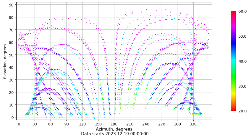
Azimuth-elevation plot for station EIVI. Signal to Noise S1C Data file EIVI00ESP_R_2023353.xtr
