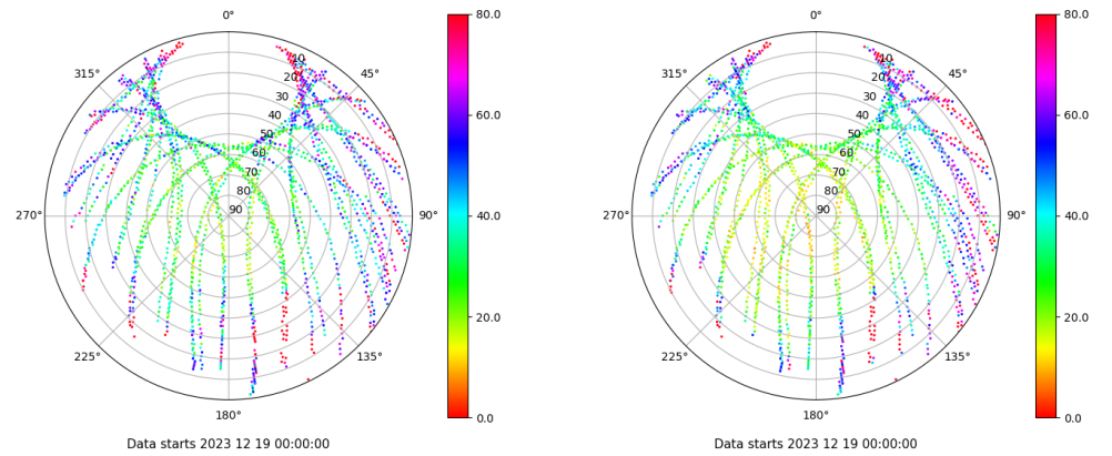
Skyplot for station EIVI. Parameter M1C Data file EIVI00ESP_R_2023353.xtr Skyplot for station EIVI. Parameter M2P Data file EIVI00ESP_R_2023353.xtr
