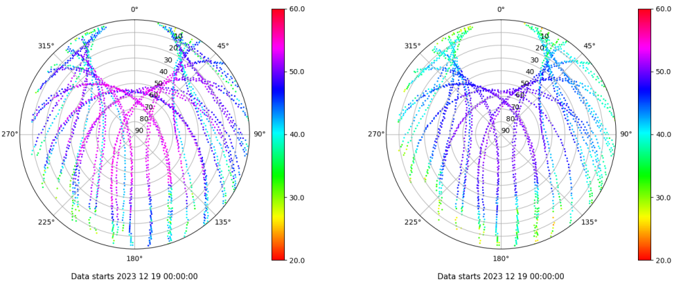
Skyplot for station EIVI. Signal to Noise S1C Data file EIVI00ESP_R_2023353.xtr Skyplot for station EIVI. Signal to Noise S2P Data file EIVI00ESP_R_2023353.xtr
