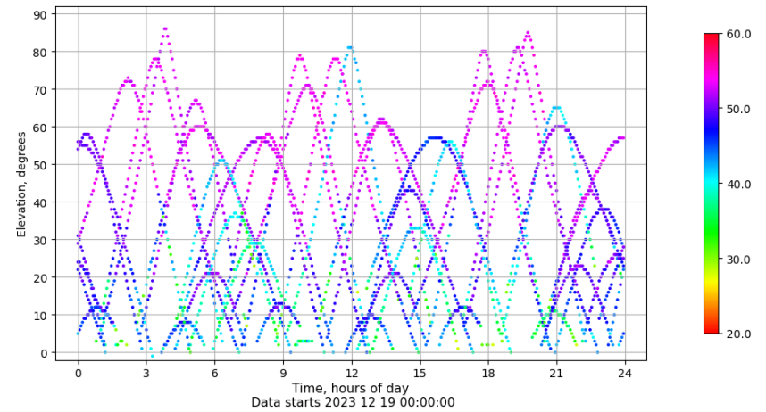
Time-elevation plot for station EIVI. Signal to Noise S1C Data file EIVI00ESP_R_2023353.xtr
