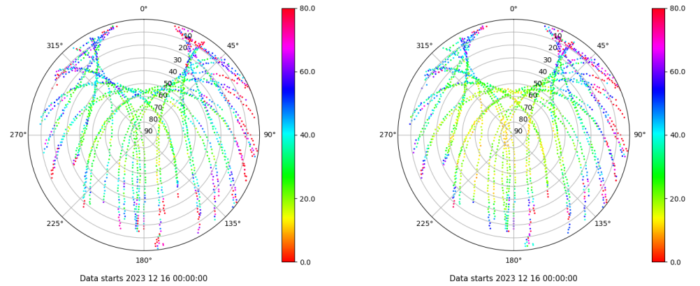
Skyplot for station EIVI. Parameter M1C Data file EIVI00ESP_R_2023350.xtr Skyplot for station EIVI. Parameter M2P Data file EIVI00ESP_R_2023350.xtr
