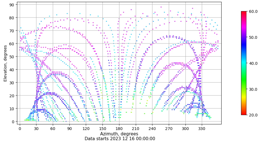
Azimuth-elevation plot for station EIVI. Signal to Noise S1C Data file EIVI00ESP_R_2023350.xtr
