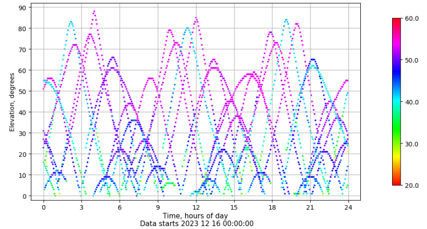
Time-elevation plot for station EIVI. Signal to Noise S1C Data file EIVI00ESP_R_2023350.xtr
