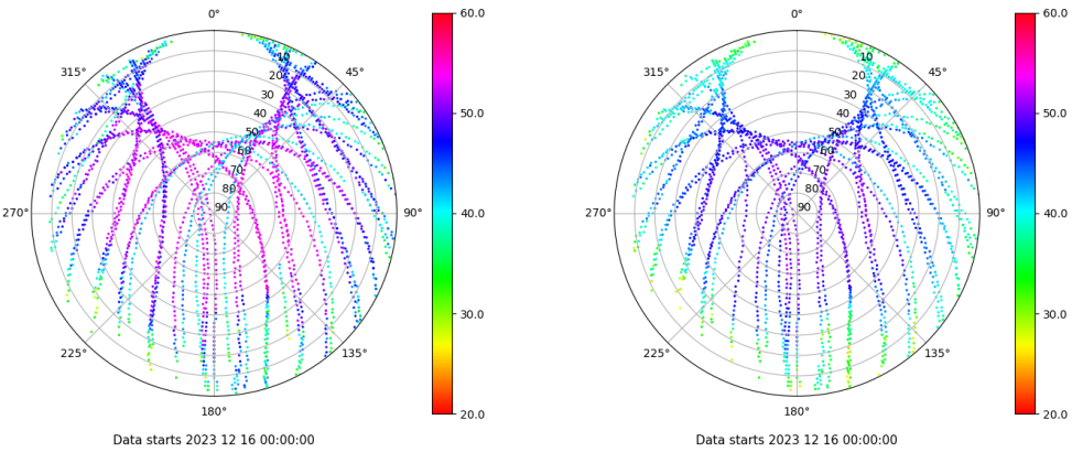
Skyplot for station EIVI. Signal to Noise S1C Data file EIVI00ESP_R_2023350.xtr Skyplot for station EIVI. Signal to Noise S2P Data file EIVI00ESP_R_2023350.xtr
