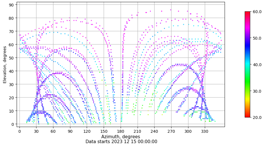
Azimuth-elevation plot for station EIVI. Signal to Noise S1C Data file EIVI00ESP_R_2023349.xtr
