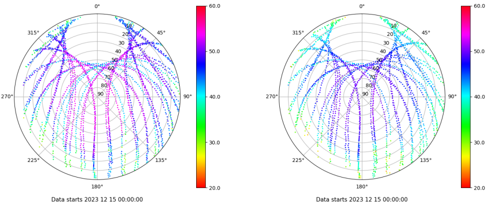
Skyplot for station EIVI. Signal to Noise S1C Data file EIVI00ESP_R_2023349.xtr Skyplot for station EIVI. Signal to Noise S2P Data file EIVI00ESP_R_2023349.xtr
