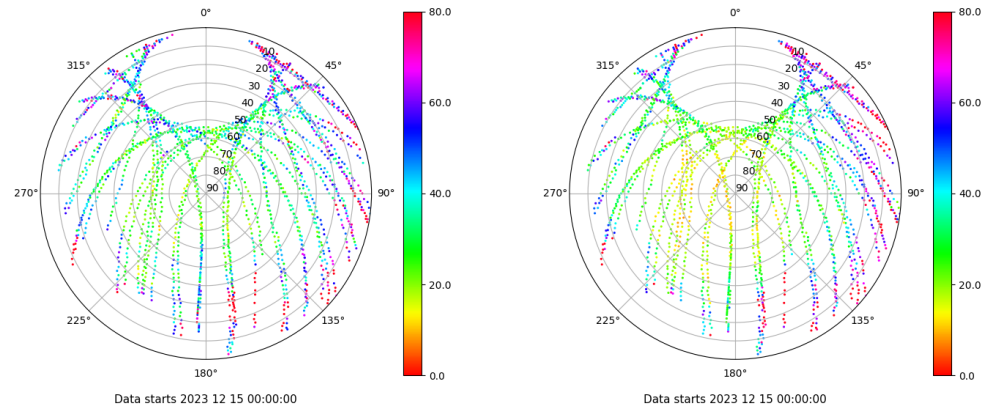
Skyplot for station EIVI. Parameter M1C Data file EIVI00ESP_R_2023349.xtr Skyplot for station EIVI. Parameter M2P Data file EIVI00ESP_R_2023349.xtr
