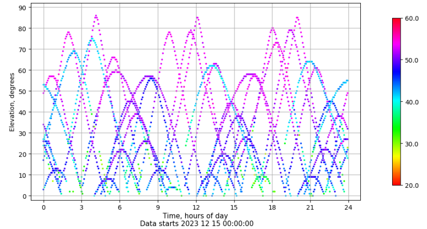
Time-elevation plot for station EIVI. Signal to Noise S1C Data file EIVI00ESP_R_2023349.xtr
