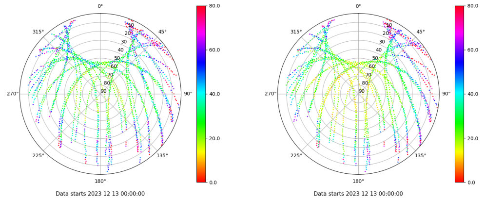
Skyplot for station EIVI. Parameter M1C Data file EIVI00ESP_R_2023347.xtr Skyplot for station EIVI. Parameter M2P Data file EIVI00ESP_R_2023347.xtr
