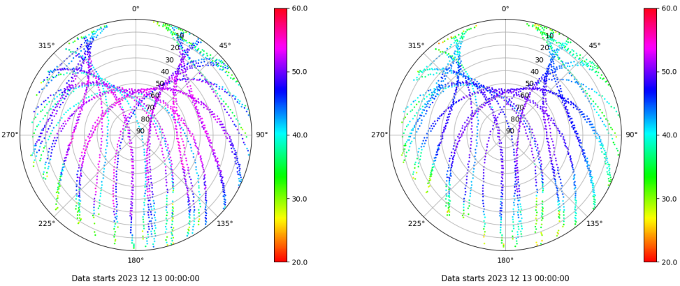
Skyplot for station EIVI. Signal to Noise S1C Data file EIVI00ESP_R_2023347.xtr Skyplot for station EIVI. Signal to Noise S2P Data file EIVI00ESP_R_2023347.xtr
