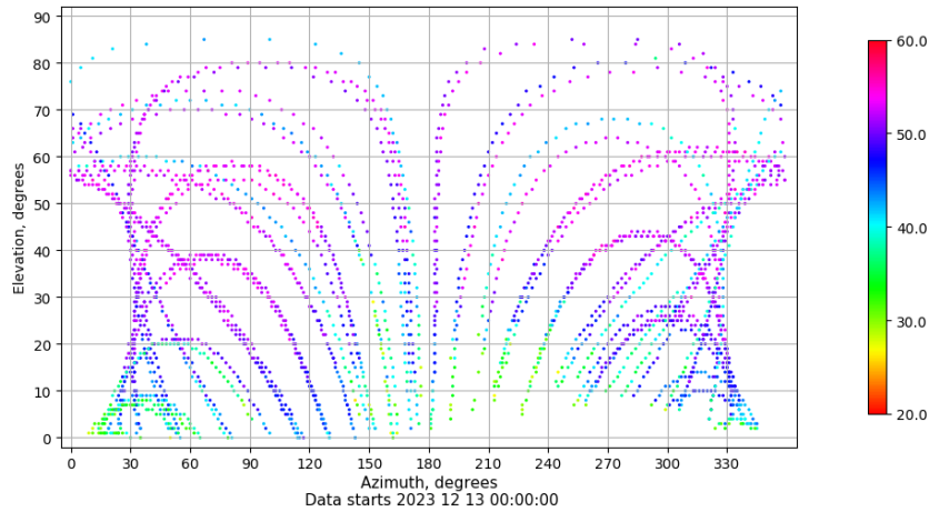
Azimuth-elevation plot for station EIVI. Signal to Noise S1C Data file EIVI00ESP_R_2023347.xtr
