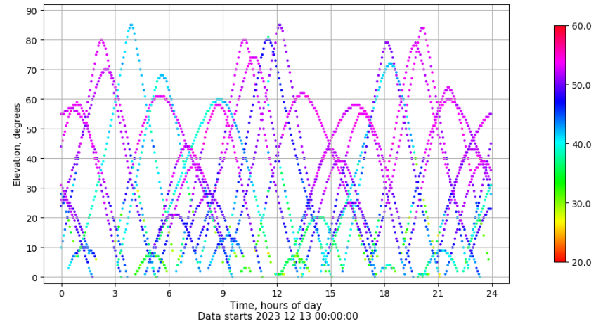
Time-elevation plot for station EIVI. Signal to Noise S1C Data file EIVI00ESP_R_2023347.xtr
