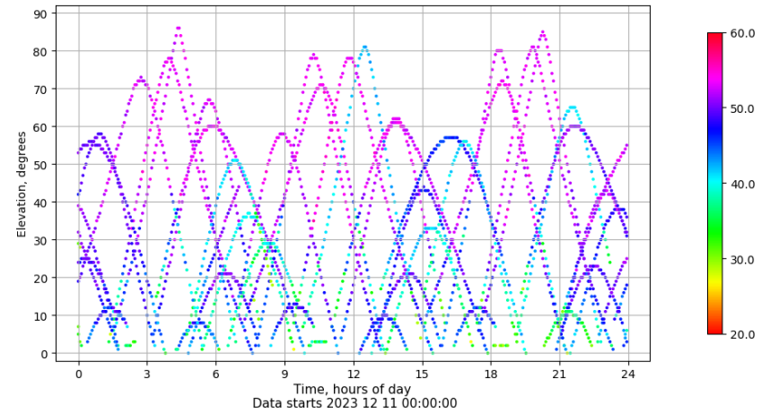
Time-elevation plot for station EIVI. Signal to Noise S1C Data file EIVI00ESP_R_2023345.xtr
