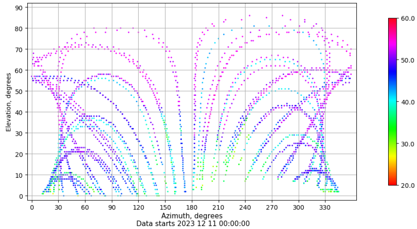
Azimuth-elevation plot for station EIVI. Signal to Noise S1C Data file EIVI00ESP_R_2023345.xtr
