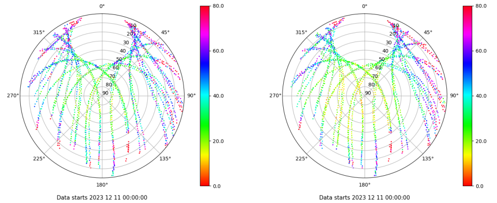
Skyplot for station EIVI. Parameter M1C Data file EIVI00ESP_R_2023345.xtr Skyplot for station EIVI. Parameter M2P Data file EIVI00ESP_R_2023345.xtr
