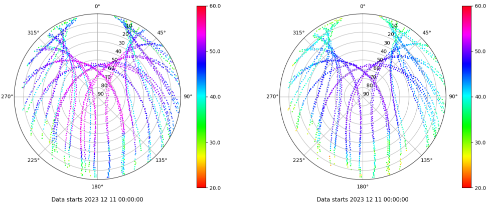
Skyplot for station EIVI. Signal to Noise S1C Data file EIVI00ESP_R_2023345.xtr Skyplot for station EIVI. Signal to Noise S2P Data file EIVI00ESP_R_2023345.xtr
