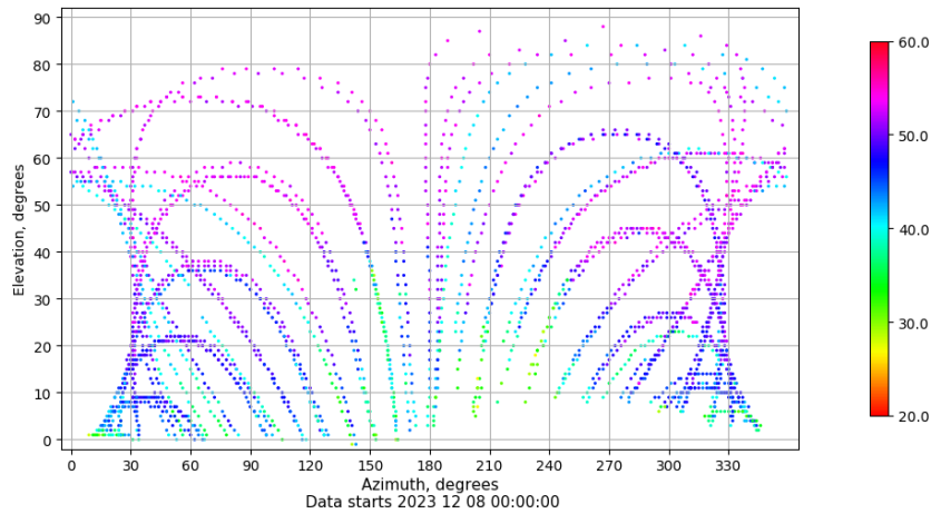
Azimuth-elevation plot for station EIVI. Signal to Noise S1C Data file EIVI00ESP_R_2023342.xtr
