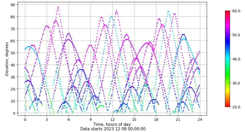
Time-elevation plot for station EIVI. Signal to Noise S1C Data file EIVI00ESP_R_2023342.xtr
