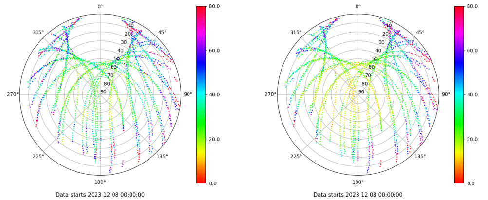
Skyplot for station EIVI. Parameter M1C Data file EIVI00ESP_R_2023342.xtr Skyplot for station EIVI. Parameter M2P Data file EIVI00ESP_R_2023342.xtr
