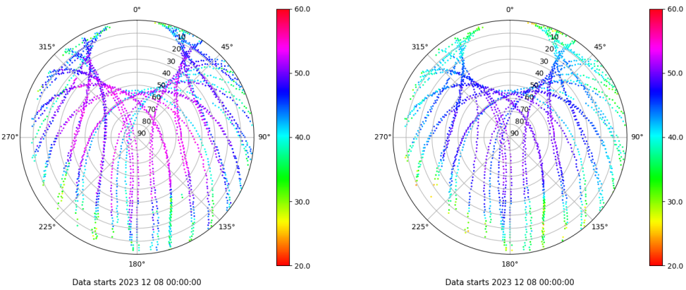
Skyplot for station EIVI. Signal to Noise S1C Data file EIVI00ESP_R_2023342.xtr Skyplot for station EIVI. Signal to Noise S2P Data file EIVI00ESP_R_2023342.xtr
