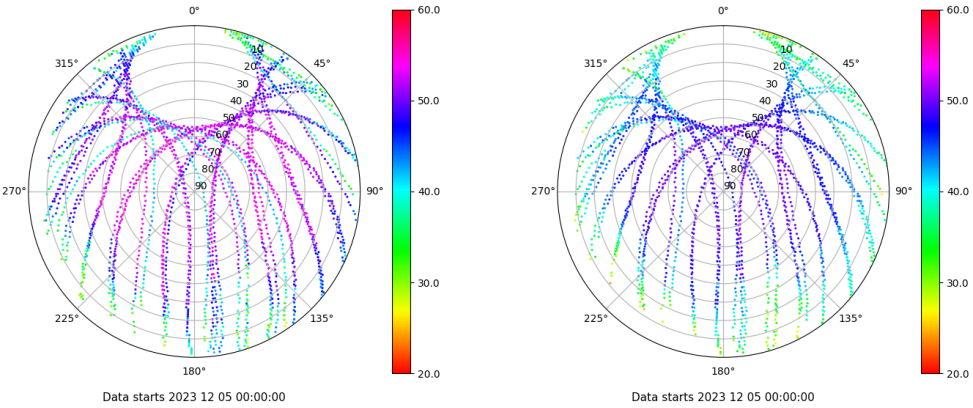
Skyplot for station EIVI. Signal to Noise S1C Data file EIVI00ESP_R_2023339.xtr Skyplot for station EIVI. Signal to Noise S2P Data file EIVI00ESP_R_2023339.xtr
