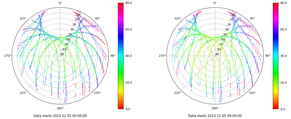
Skyplot for station EIVI. Parameter M1C Data file EIVI00ESP_R_2023339.xtr Skyplot for station EIVI. Parameter M2P Data file EIVI00ESP_R_2023339.xtr
