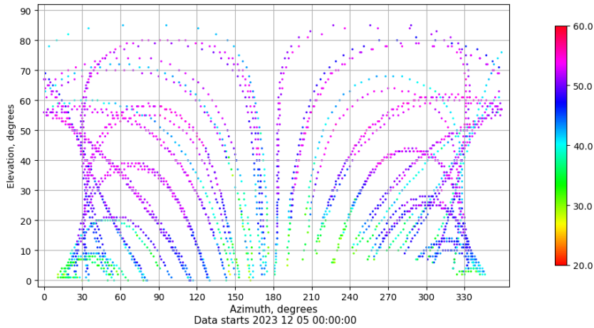
Azimuth-elevation plot for station EIVI. Signal to Noise S1C Data file EIVI00ESP_R_2023339.xtr
