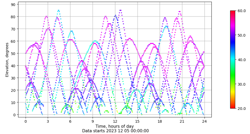
Time-elevation plot for station EIVI. Signal to Noise S1C Data file EIVI00ESP_R_2023339.xtr
