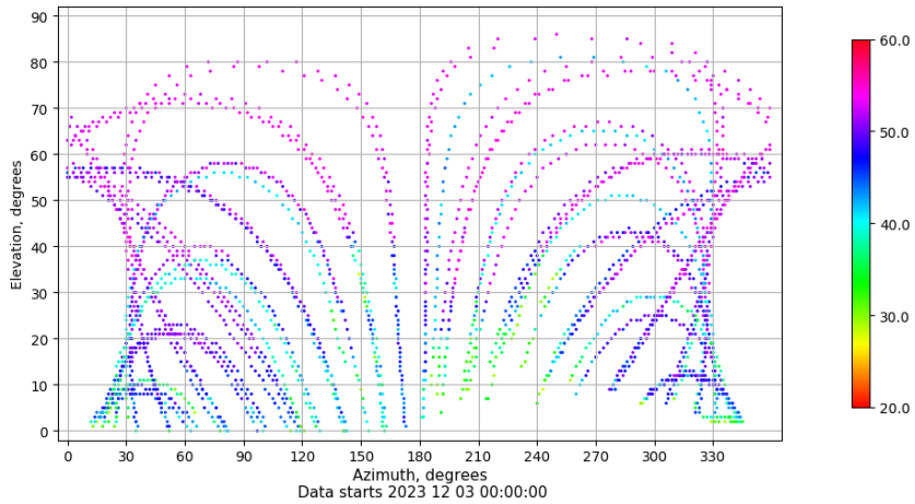
Azimuth-elevation plot for station EIVI. Signal to Noise S1C Data file EIVI00ESP_R_2023337.xtr
