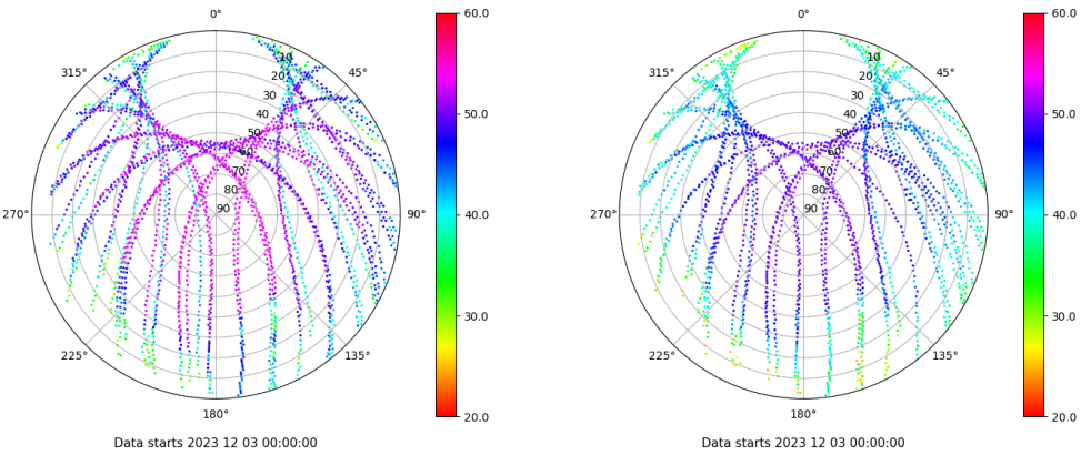
Skyplot for station EIVI. Signal to Noise S1C Data file EIVI00ESP_R_2023337.xtr Skyplot for station EIVI. Signal to Noise S2P Data file EIVI00ESP_R_2023337.xtr
