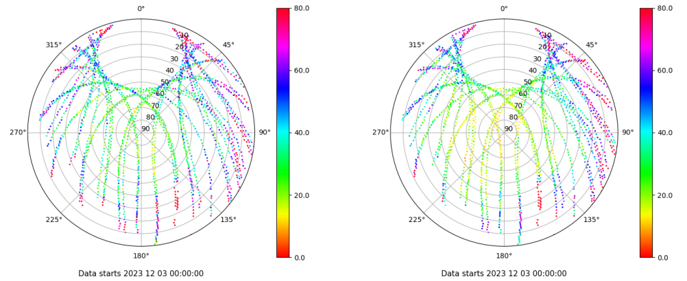
Skyplot for station EIVI. Parameter M1C Data file EIVI00ESP_R_2023337.xtr Skyplot for station EIVI. Parameter M2P Data file EIVI00ESP_R_2023337.xtr
