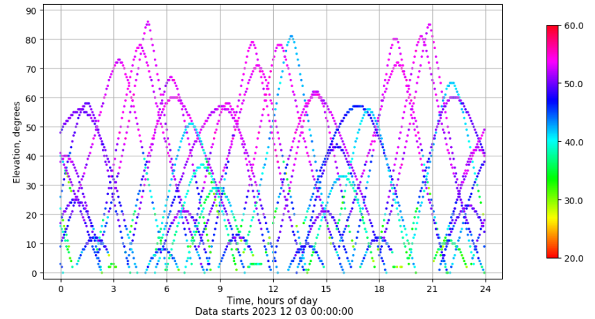
Time-elevation plot for station EIVI. Signal to Noise S1C Data file EIVI00ESP_R_2023337.xtr
