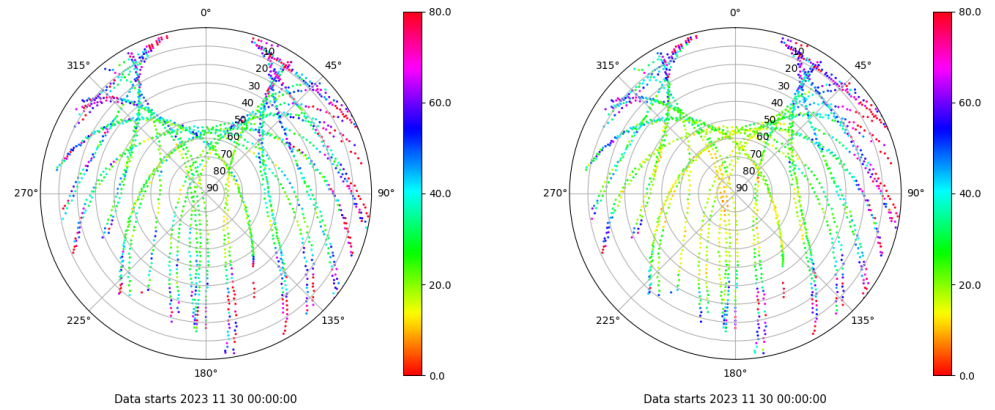
Skyplot for station EIVI. Parameter M1C Data file EIVI00ESP_R_2023334.xtr Skyplot for station EIVI. Parameter M2P Data file EIVI00ESP_R_2023334.xtr
