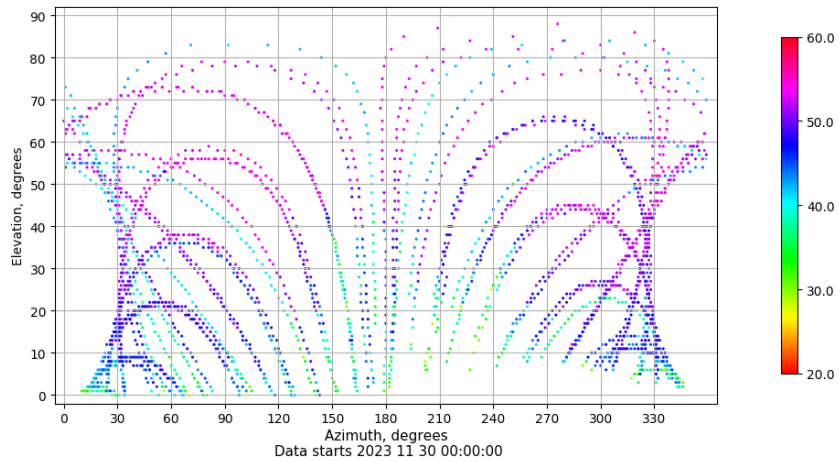
Azimuth-elevation plot for station EIVI. Signal to Noise S1C Data file EIVI00ESP_R_2023334.xtr
