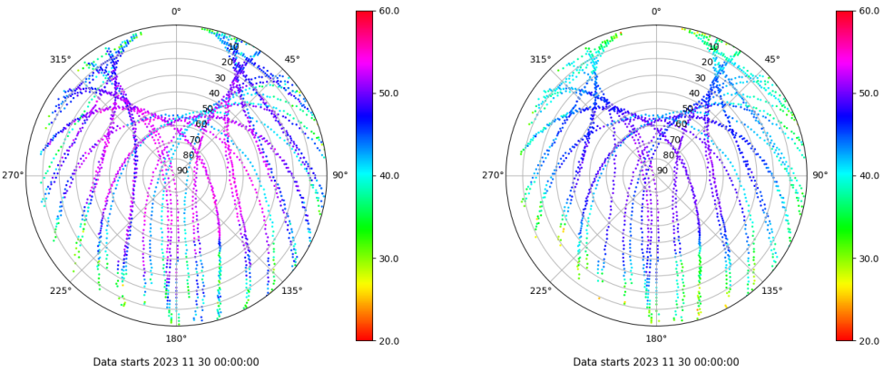
Skyplot for station EIVI. Signal to Noise S1C Data file EIVI00ESP_R_2023334.xtr Skyplot for station EIVI. Signal to Noise S2P Data file EIVI00ESP_R_2023334.xtr
