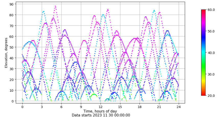
Time-elevation plot for station EIVI. Signal to Noise S1C Data file EIVI00ESP_R_2023334.xtr
