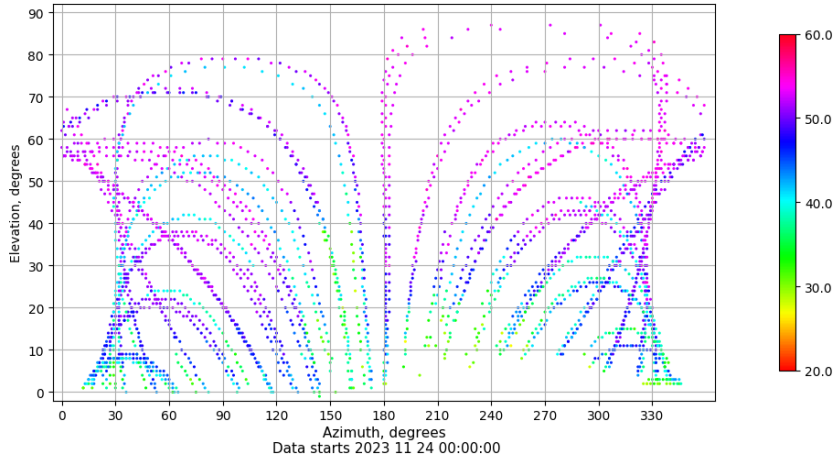
Azimuth-elevation plot for station EIVI. Signal to Noise S1C Data file EIVI00ESP_R_2023328.xtr
