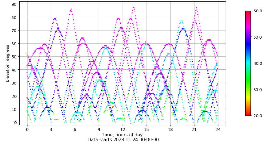
Time-elevation plot for station EIVI. Signal to Noise S1C Data file EIVI00ESP_R_2023328.xtr
