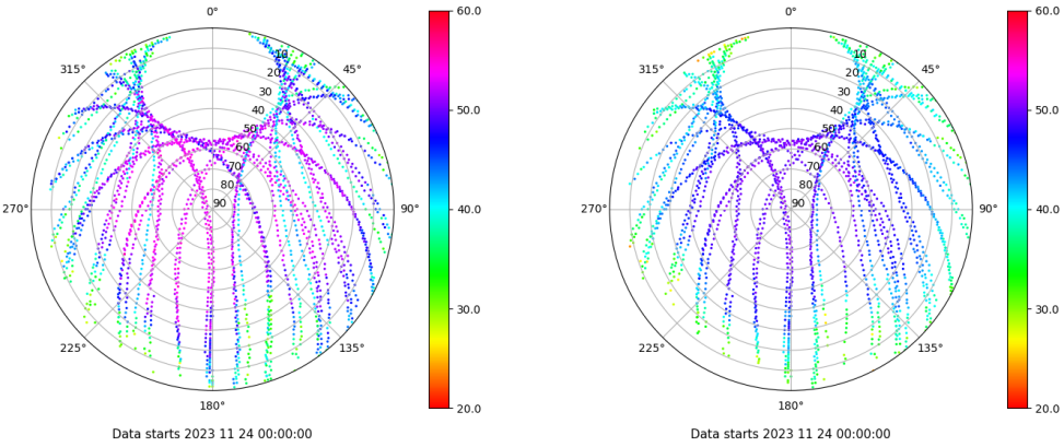
Skyplot for station EIVI. Signal to Noise S1C Data file EIVI00ESP_R_2023328.xtr Skyplot for station EIVI. Signal to Noise S2P Data file EIVI00ESP_R_2023328.xtr
