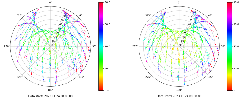
Skyplot for station EIVI. Parameter M1C Data file EIVI00ESP_R_2023328.xtr Skyplot for station EIVI. Parameter M2P Data file EIVI00ESP_R_2023328.xtr
