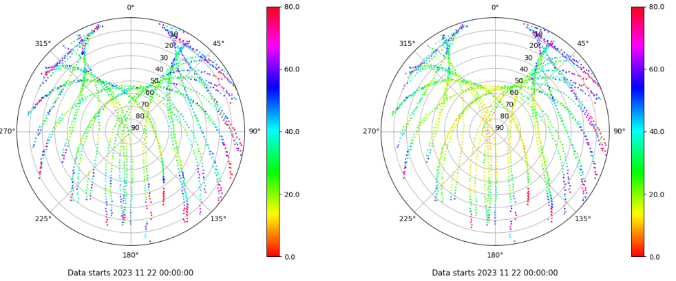
Skyplot for station EIVI. Parameter M1C Data file EIVI00ESP_R_2023326.xtr Skyplot for station EIVI. Parameter M2P Data file EIVI00ESP_R_2023326.xtr
