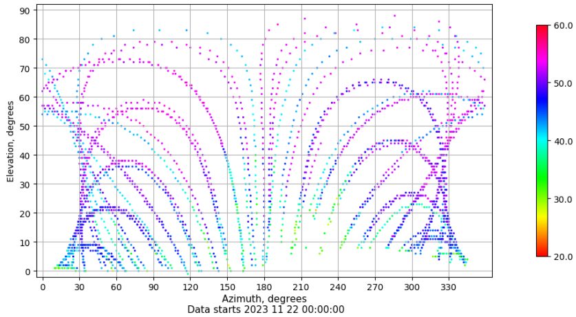
Azimuth-elevation plot for station EIVI. Signal to Noise S1C Data file EIVI00ESP_R_2023326.xtr
