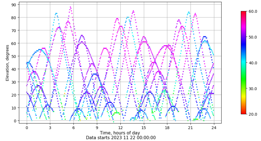
Time-elevation plot for station EIVI. Signal to Noise S1C Data file EIVI00ESP_R_2023326.xtr
