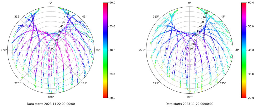
Skyplot for station EIVI. Signal to Noise S1C Data file EIVI00ESP_R_2023326.xtr Skyplot for station EIVI. Signal to Noise S2P Data file EIVI00ESP_R_2023326.xtr
