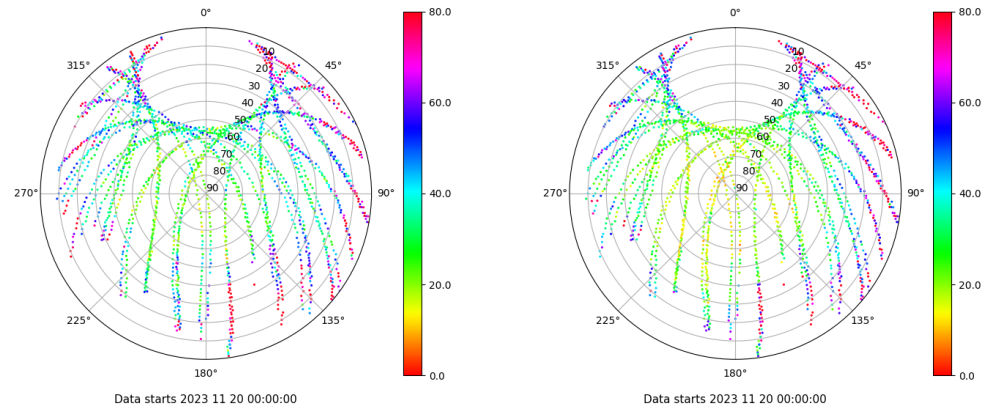
Skyplot for station EIVI. Parameter M1C Data file EIVI00ESP_R_2023324.xtr Skyplot for station EIVI. Parameter M2P Data file EIVI00ESP_R_2023324.xtr
