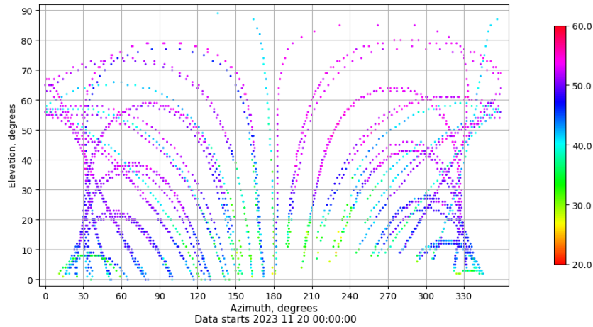
Azimuth-elevation plot for station EIVI. Signal to Noise S1C Data file EIVI00ESP_R_2023324.xtr
