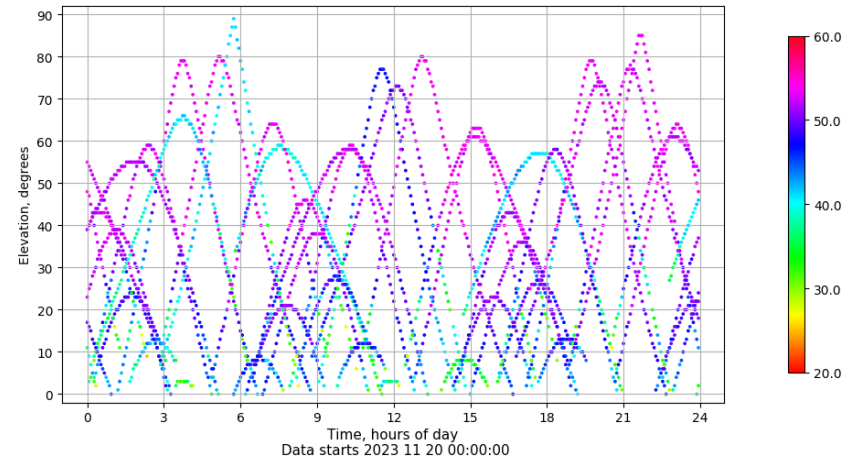
Time-elevation plot for station EIVI. Signal to Noise S1C Data file EIVI00ESP_R_2023324.xtr
