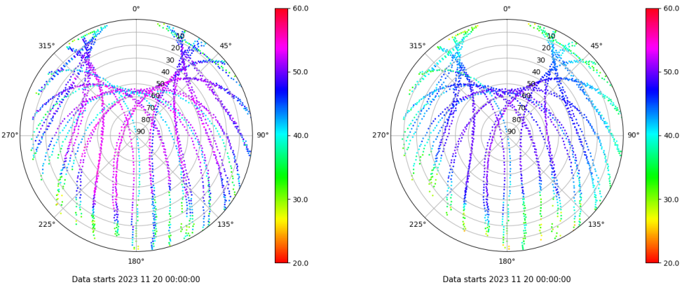
Skyplot for station EIVI. Signal to Noise S1C Data file EIVI00ESP_R_2023324.xtr Skyplot for station EIVI. Signal to Noise S2P Data file EIVI00ESP_R_2023324.xtr
