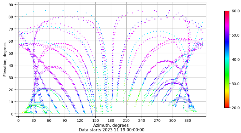
Azimuth-elevation plot for station EIVI. Signal to Noise S1C Data file EIVI00ESP_R_2023323.xtr
