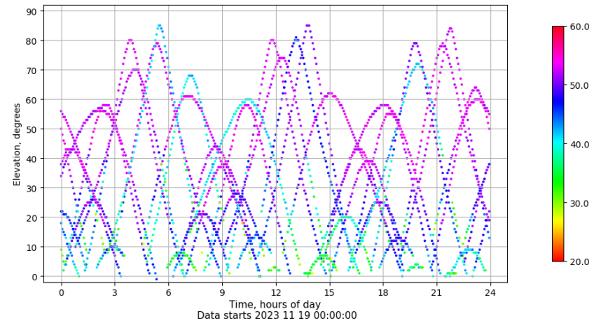
Time-elevation plot for station EIVI. Signal to Noise S1C Data file EIVI00ESP_R_2023323.xtr
