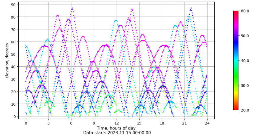
Time-elevation plot for station EIVI. Signal to Noise S1C Data file EIVI00ESP_R_2023319.xtr
