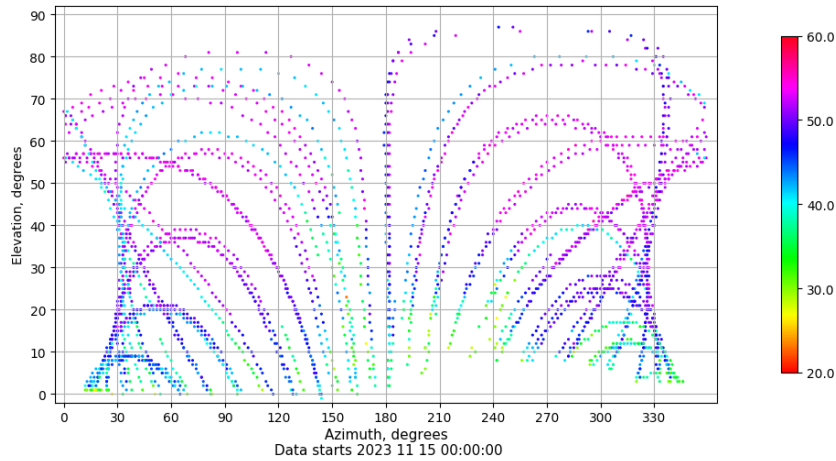
Azimuth-elevation plot for station EIVI. Signal to Noise S1C Data file EIVI00ESP_R_2023319.xtr
