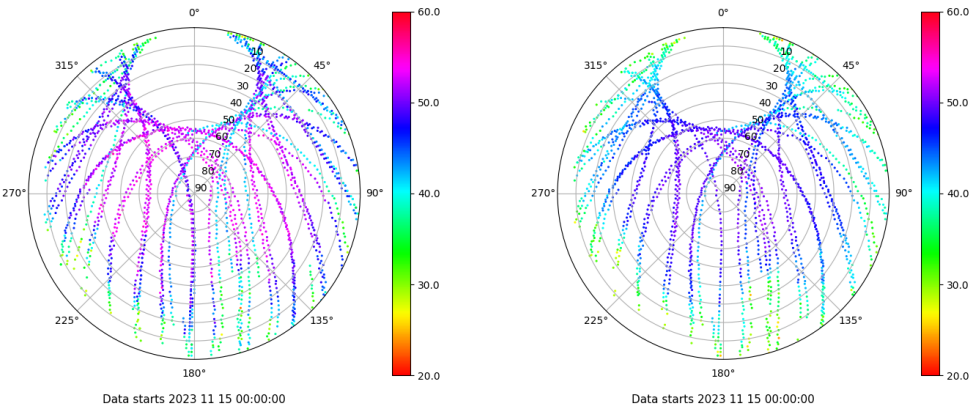
Skyplot for station EIVI. Signal to Noise S1C Data file EIVI00ESP_R_2023319.xtr Skyplot for station EIVI. Signal to Noise S2P Data file EIVI00ESP_R_2023319.xtr
