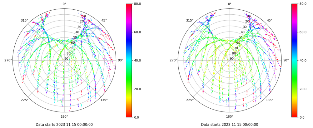
Skyplot for station EIVI. Parameter M1C Data file EIVI00ESP_R_2023319.xtr Skyplot for station EIVI. Parameter M2P Data file EIVI00ESP_R_2023319.xtr
