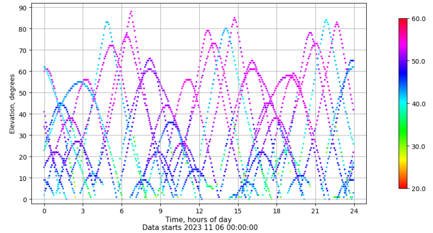
Time-elevation plot for station EIVI. Signal to Noise S1C Data file EIVI00ESP_R_2023310.xtr
