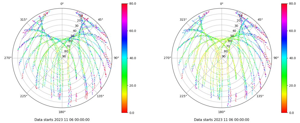
Skyplot for station EIVI. Parameter M1C Data file EIVI00ESP_R_2023310.xtr Skyplot for station EIVI. Parameter M2P Data file EIVI00ESP_R_2023310.xtr
