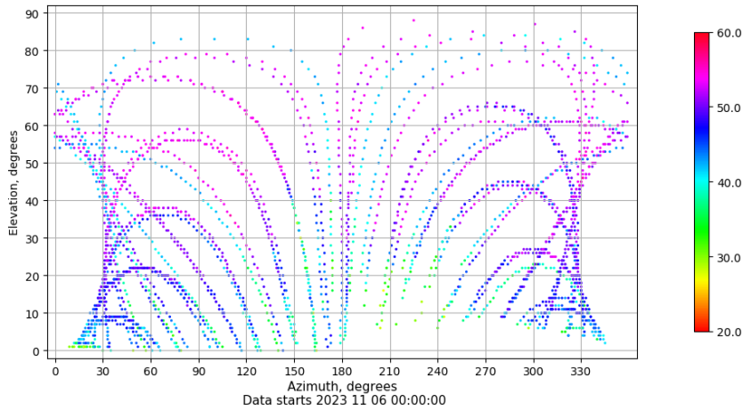
Azimuth-elevation plot for station EIVI. Signal to Noise S1C Data file EIVI00ESP_R_2023310.xtr
