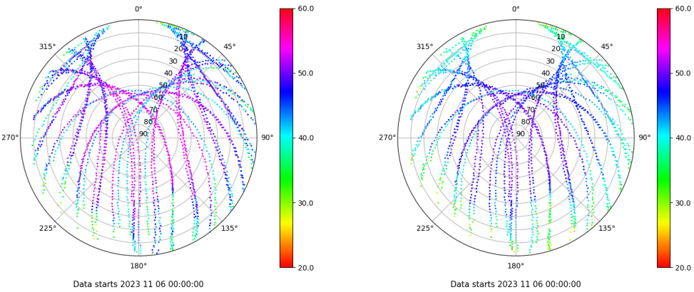
Skyplot for station EIVI. Signal to Noise S1C Data file EIVI00ESP_R_2023310.xtr Skyplot for station EIVI. Signal to Noise S2P Data file EIVI00ESP_R_2023310.xtr
