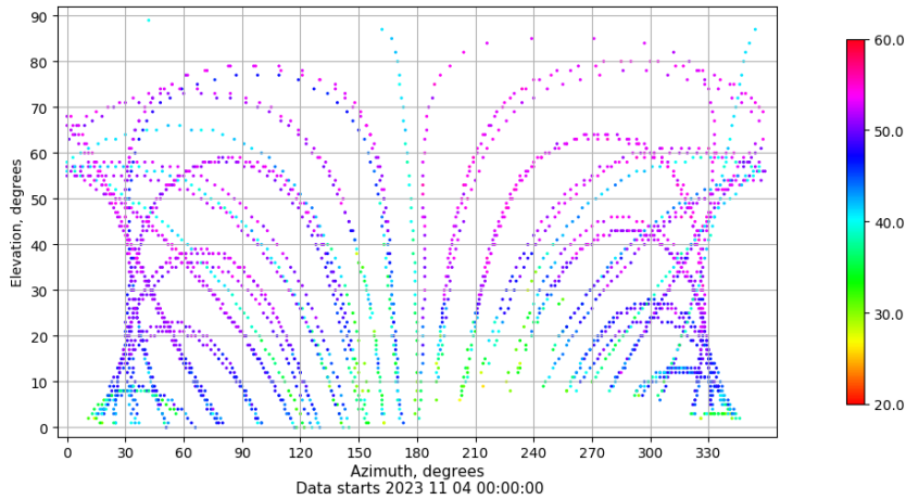
Azimuth-elevation plot for station EIVI. Signal to Noise S1C Data file EIVI00ESP_R_2023308.xtr
