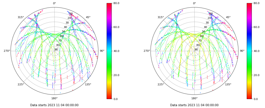
Skyplot for station EIVI. Parameter M1C Data file EIVI00ESP_R_2023308.xtr Skyplot for station EIVI. Parameter M2P Data file EIVI00ESP_R_2023308.xtr
