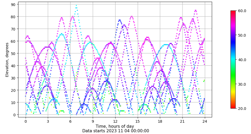
Time-elevation plot for station EIVI. Signal to Noise S1C Data file EIVI00ESP_R_2023308.xtr
