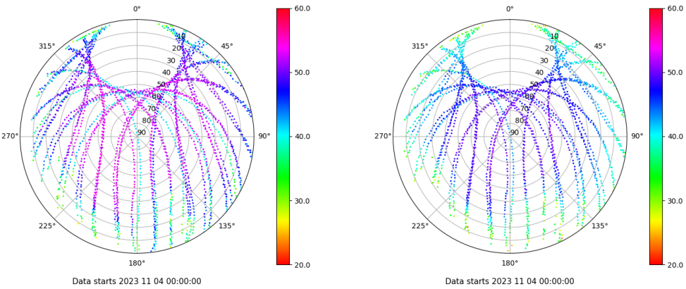
Skyplot for station EIVI. Signal to Noise S1C Data file EIVI00ESP_R_2023308.xtr Skyplot for station EIVI. Signal to Noise S2P Data file EIVI00ESP_R_2023308.xtr
