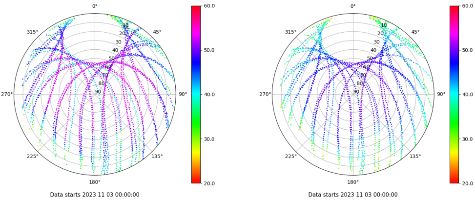
Skyplot for station EIVI. Signal to Noise S1C Data file EIVI00ESP_R_2023307.xtr Skyplot for station EIVI. Signal to Noise S2P Data file EIVI00ESP_R_2023307.xtr
