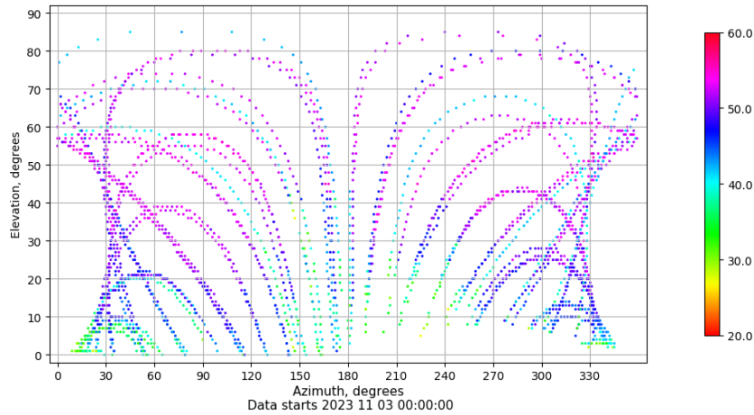
Azimuth-elevation plot for station EIVI. Signal to Noise S1C Data file EIVI00ESP_R_2023307.xtr
