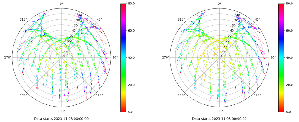
Skyplot for station EIVI. Parameter M1C Data file EIVI00ESP_R_2023307.xtr Skyplot for station EIVI. Parameter M2P Data file EIVI00ESP_R_2023307.xtr
