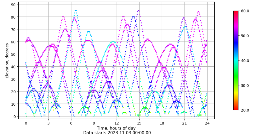
Time-elevation plot for station EIVI. Signal to Noise S1C Data file EIVI00ESP_R_2023307.xtr
