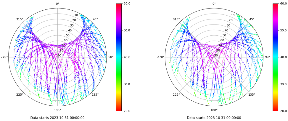
Skyplot for station EIVI. Signal to Noise S1C Data file EIVI00ESP_R_2023304.xtr Skyplot for station EIVI. Signal to Noise S2S Data file EIVI00ESP_R_2023304.xtr
