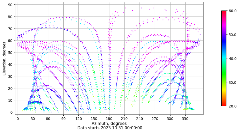
Azimuth-elevation plot for station EIVI. Signal to Noise S1C Data file EIVI00ESP_R_2023304.xtr
