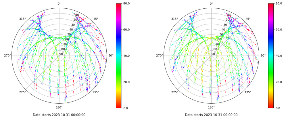
Skyplot for station EIVI. Parameter M1C Data file EIVI00ESP_R_2023304.xtr Skyplot for station EIVI. Parameter M2P Data file EIVI00ESP_R_2023304.xtr
