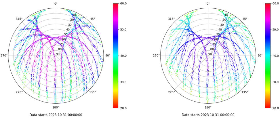
Skyplot for station EIVI. Signal to Noise S1C Data file EIVI00ESP_R_2023304.xtr Skyplot for station EIVI. Signal to Noise S2P Data file EIVI00ESP_R_2023304.xtr
