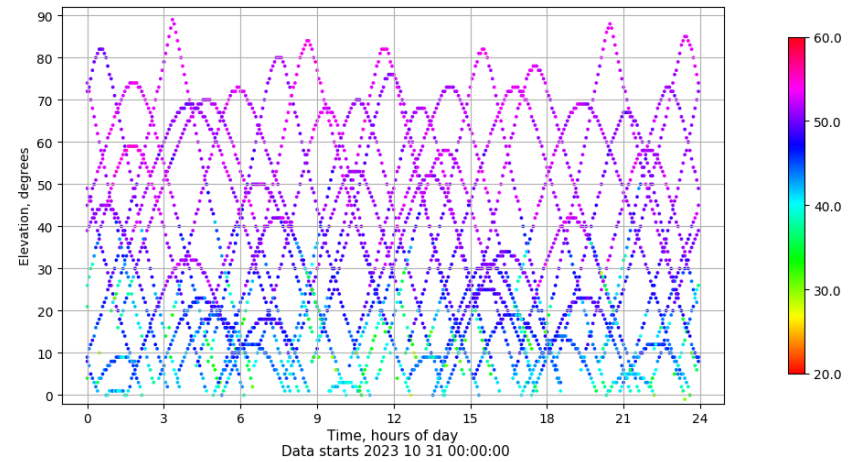
Time-elevation plot for station EIVI. Signal to Noise S1C Data file EIVI00ESP_R_2023304.xtr
