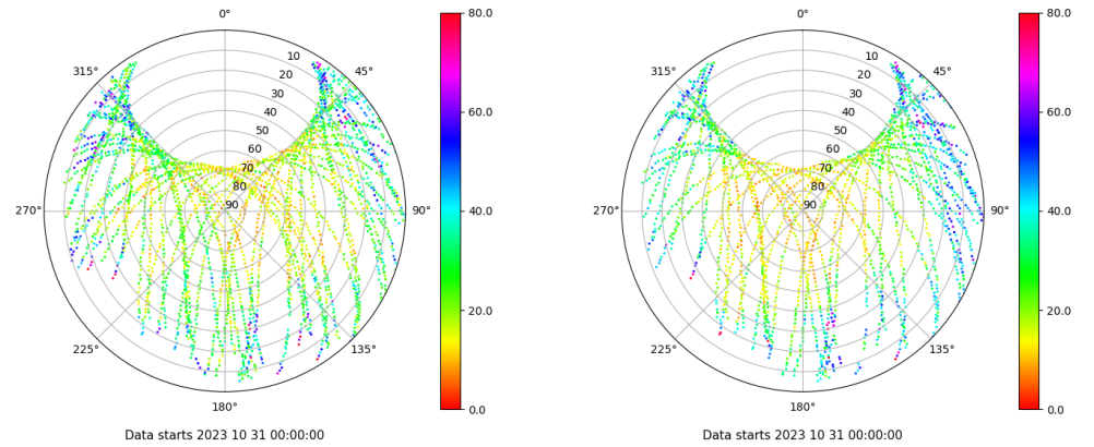
Skyplot for station EIVI. Parameter M1C Data file EIVI00ESP_R_2023304.xtr Skyplot for station EIVI. Parameter M2S Data file EIVI00ESP_R_2023304.xtr
