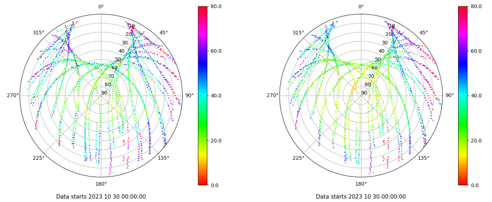
Skyplot for station EIVI. Parameter M1C Data file EIVI00ESP_R_2023303.xtr Skyplot for station EIVI. Parameter M2P Data file EIVI00ESP_R_2023303.xtr
