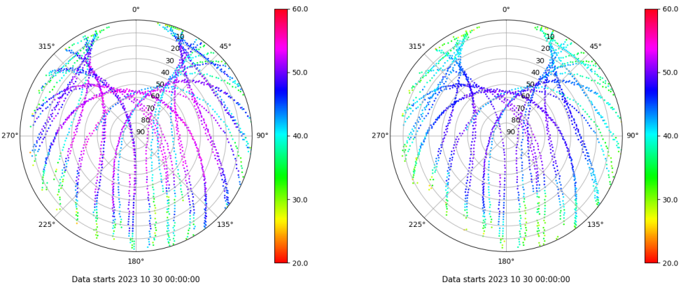
Skyplot for station EIVI. Signal to Noise S1C Data file EIVI00ESP_R_2023303.xtr Skyplot for station EIVI. Signal to Noise S2P Data file EIVI00ESP_R_2023303.xtr
