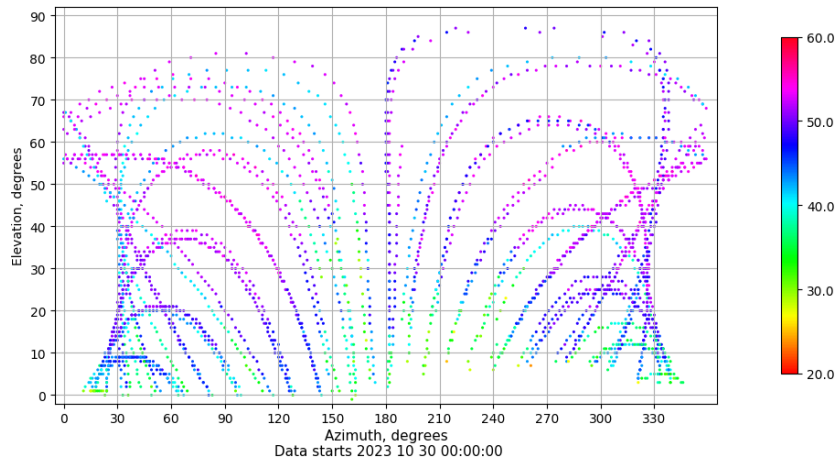
Azimuth-elevation plot for station EIVI. Signal to Noise S1C Data file EIVI00ESP_R_2023303.xtr
