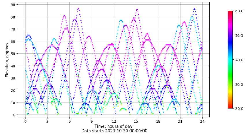
Time-elevation plot for station EIVI. Signal to Noise S1C Data file EIVI00ESP_R_2023303.xtr
