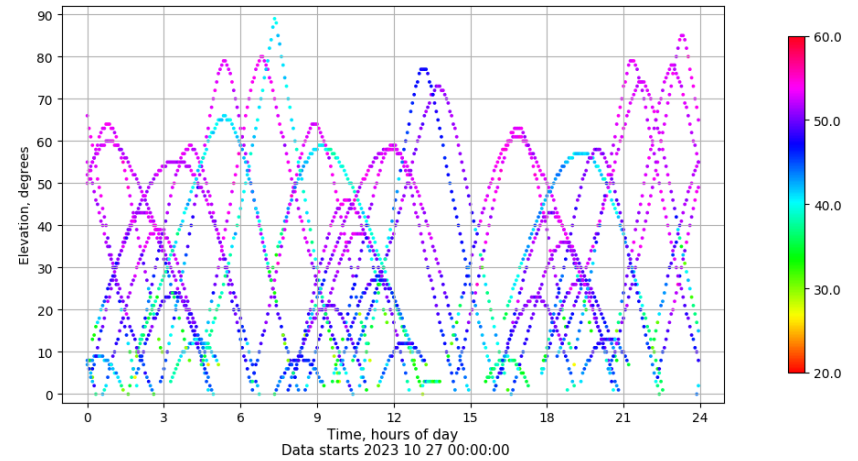
Time-elevation plot for station EIVI. Signal to Noise S1C Data file EIVI00ESP_R_2023300.xtr
