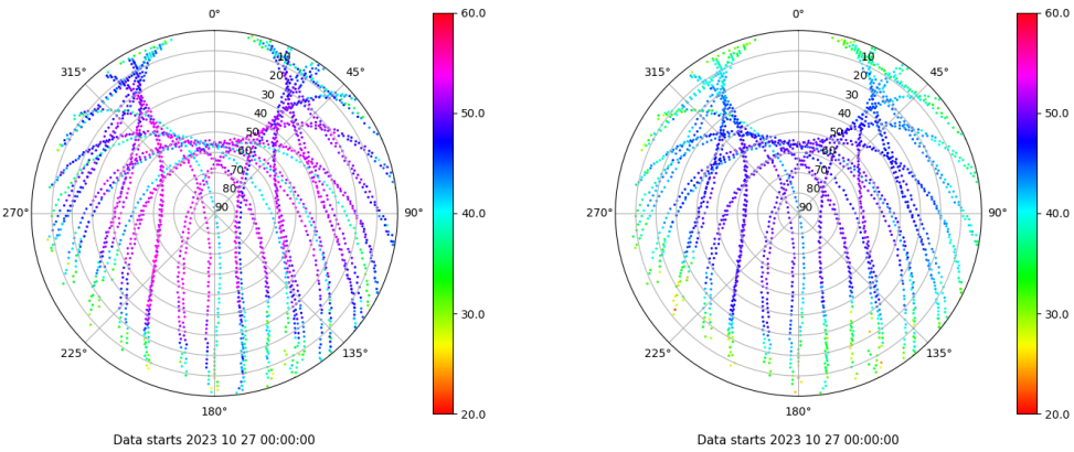
Skyplot for station EIVI. Signal to Noise S1C Data file EIVI00ESP_R_2023300.xtr Skyplot for station EIVI. Signal to Noise S2P Data file EIVI00ESP_R_2023300.xtr
