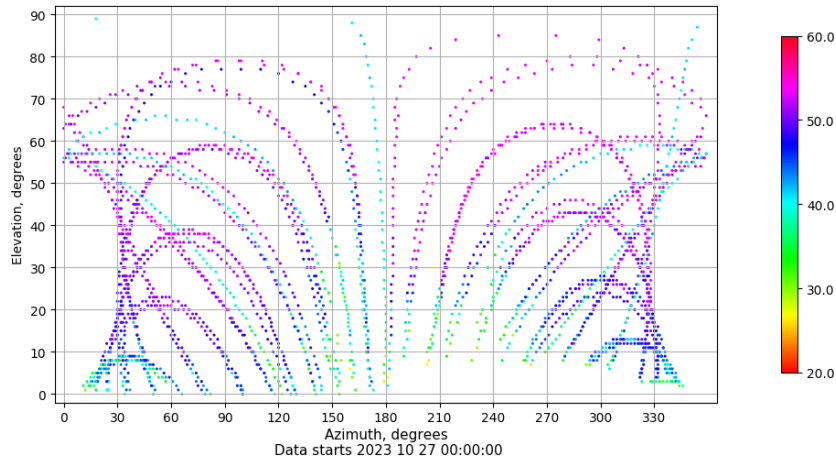
Azimuth-elevation plot for station EIVI. Signal to Noise S1C Data file EIVI00ESP_R_2023300.xtr
