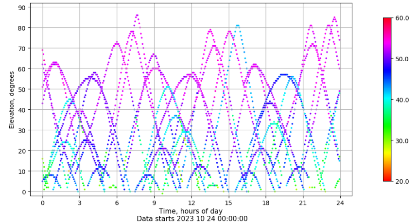
Time-elevation plot for station EIVI. Signal to Noise S1C Data file EIVI00ESP_R_2023297.xtr
