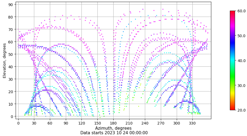
Azimuth-elevation plot for station EIVI. Signal to Noise S1C Data file EIVI00ESP_R_2023297.xtr
