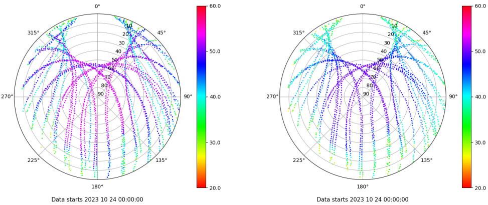
Skyplot for station EIVI. Signal to Noise S1C Data file EIVI00ESP_R_2023297.xtr Skyplot for station EIVI. Signal to Noise S2P Data file EIVI00ESP_R_2023297.xtr
