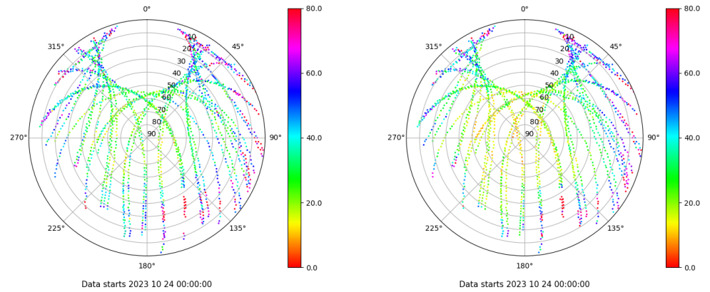
Skyplot for station EIVI. Parameter M1C Data file EIVI00ESP_R_2023297.xtr Skyplot for station EIVI. Parameter M2P Data file EIVI00ESP_R_2023297.xtr
