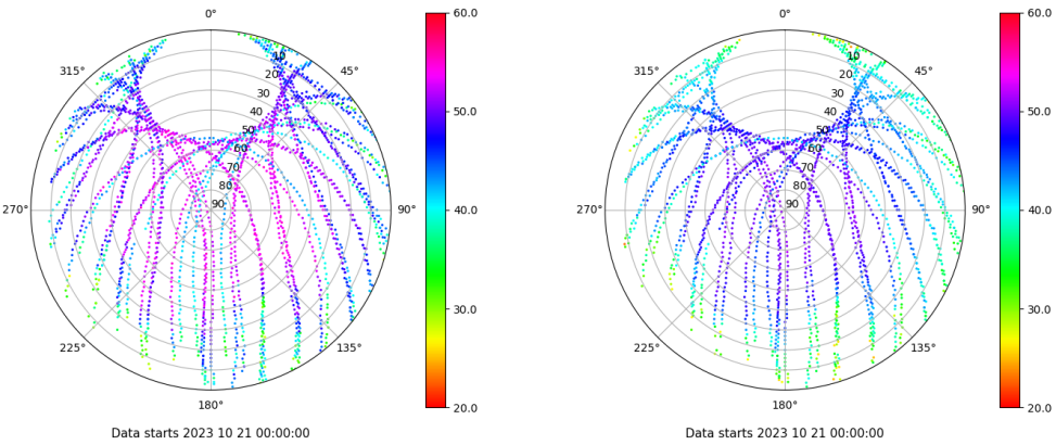
Skyplot for station EIVI. Signal to Noise S1C Data file EIVI00ESP_R_2023294.xtr Skyplot for station EIVI. Signal to Noise S2P Data file EIVI00ESP_R_2023294.xtr
