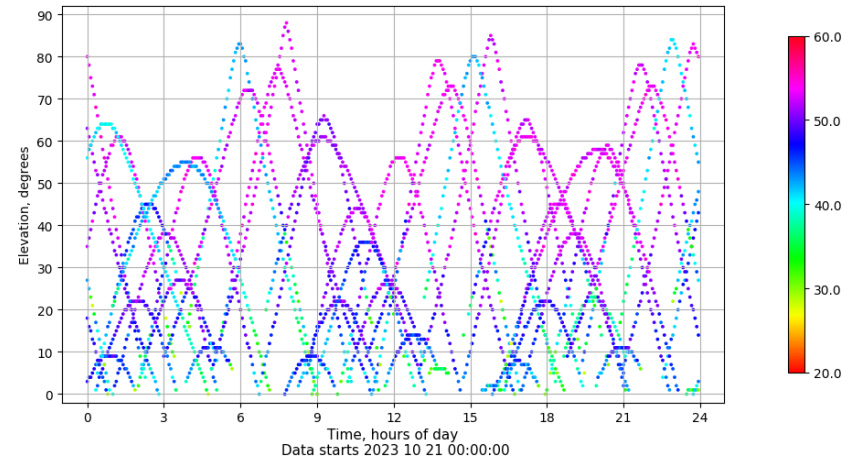
Time-elevation plot for station EIVI. Signal to Noise S1C Data file EIVI00ESP_R_2023294.xtr
