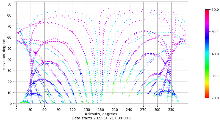
Azimuth-elevation plot for station EIVI. Signal to Noise S1C Data file EIVI00ESP_R_2023294.xtr
