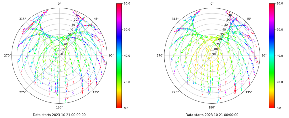
Skyplot for station EIVI. Parameter M1C Data file EIVI00ESP_R_2023294.xtr Skyplot for station EIVI. Parameter M2P Data file EIVI00ESP_R_2023294.xtr
