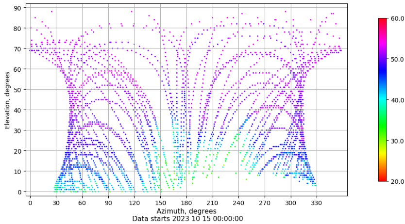
Azimuth-elevation plot for station EIVI. Signal to Noise S1C Data file EIVI00ESP_R_2023288.xtr
