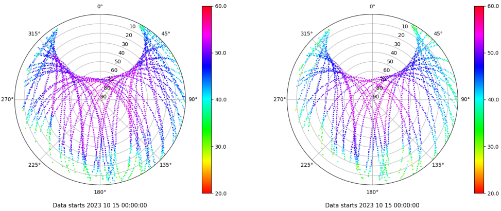
Skyplot for station EIVI. Signal to Noise S1C Data file EIVI00ESP_R_2023288.xtr Skyplot for station EIVI. Signal to Noise S2S Data file EIVI00ESP_R_2023288.xtr
