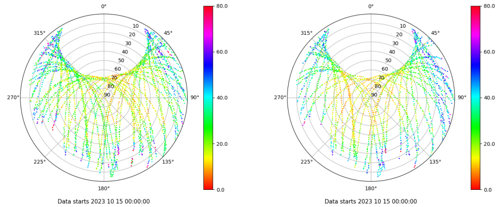
Skyplot for station EIVI. Parameter M1C Data file EIVI00ESP_R_2023288.xtr Skyplot for station EIVI. Parameter M2S Data file EIVI00ESP_R_2023288.xtr
