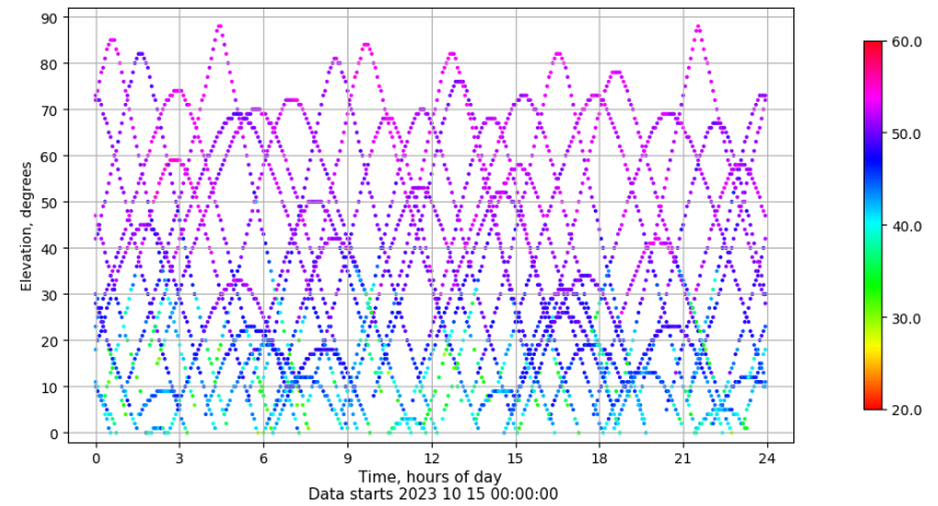
Time-elevation plot for station EIVI. Signal to Noise S1C Data file EIVI00ESP_R_2023288.xtr
