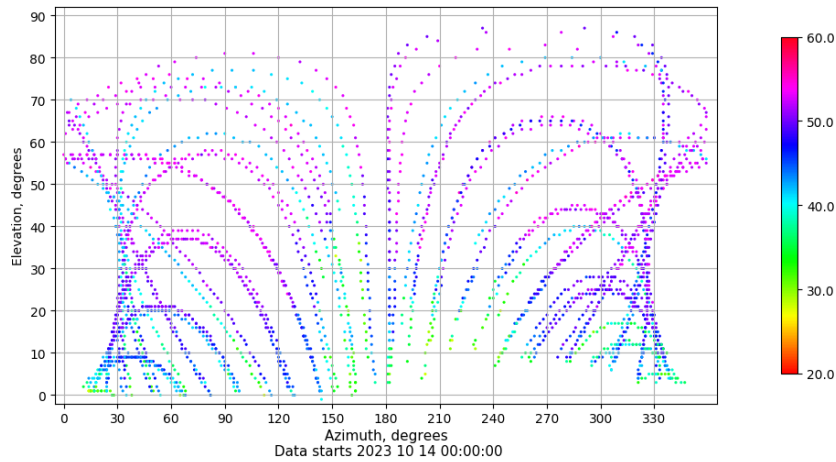
Azimuth-elevation plot for station EIVI. Signal to Noise S1C Data file EIVI00ESP_R_2023287.xtr
