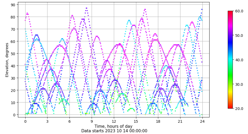
Time-elevation plot for station EIVI. Signal to Noise S1C Data file EIVI00ESP_R_2023287.xtr
