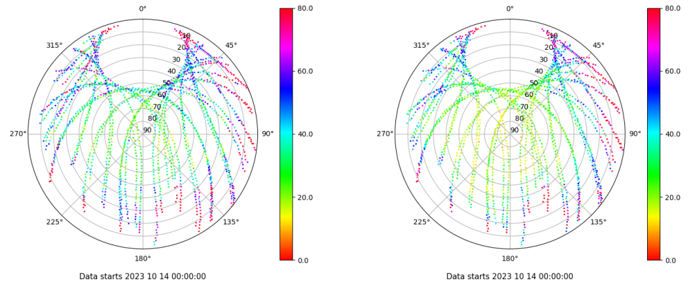
Skyplot for station EIVI. Parameter M1C Data file EIVI00ESP_R_2023287.xtr Skyplot for station EIVI. Parameter M2P Data file EIVI00ESP_R_2023287.xtr
