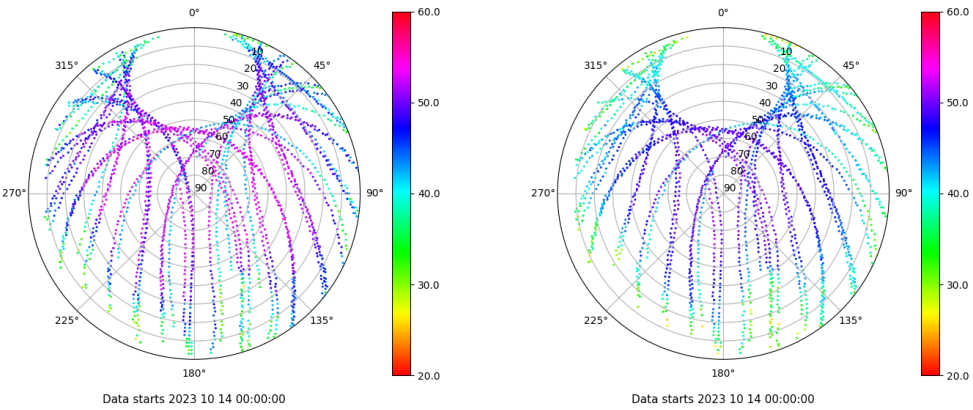
Skyplot for station EIVI. Signal to Noise S1C Data file EIVI00ESP_R_2023287.xtr Skyplot for station EIVI. Signal to Noise S2P Data file EIVI00ESP_R_2023287.xtr
