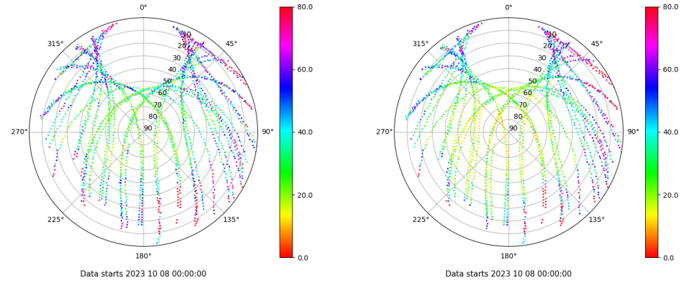
Skyplot for station EIVI. Parameter M1C Data file EIVI00ESP_R_2023281.xtr Skyplot for station EIVI. Parameter M2P Data file EIVI00ESP_R_2023281.xtr
