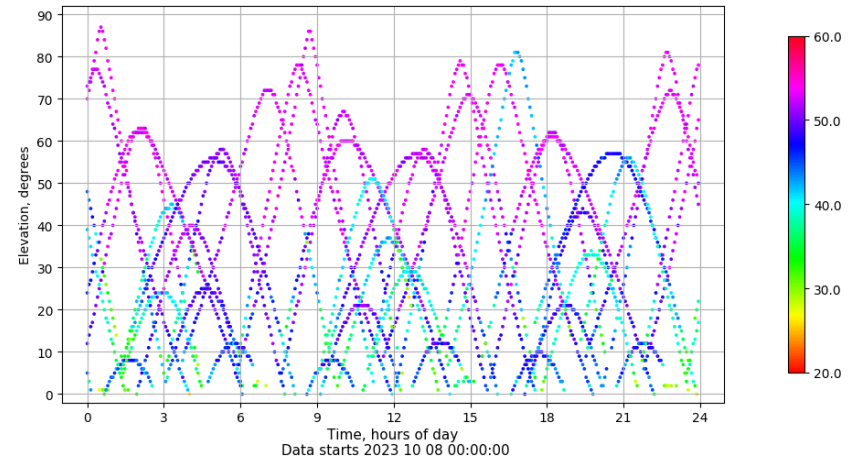
Time-elevation plot for station EIVI. Signal to Noise S1C Data file EIVI00ESP_R_2023281.xtr
