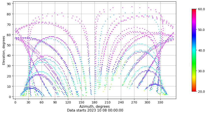
Azimuth-elevation plot for station EIVI. Signal to Noise S1C Data file EIVI00ESP_R_2023281.xtr
