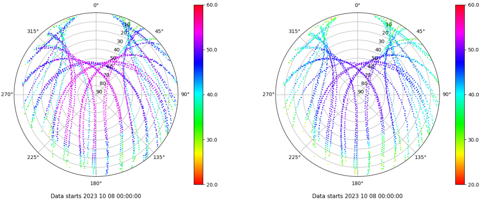
Skyplot for station EIVI. Signal to Noise S1C Data file EIVI00ESP_R_2023281.xtr Skyplot for station EIVI. Signal to Noise S2P Data file EIVI00ESP_R_2023281.xtr
