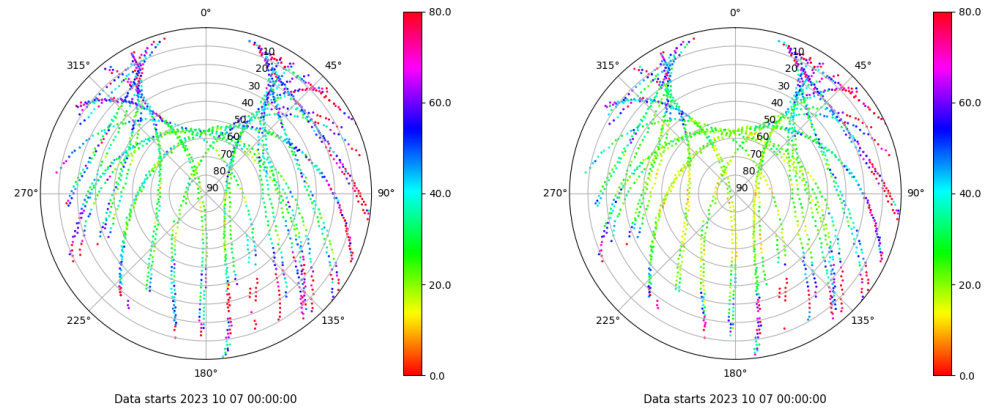
Skyplot for station EIVI. Parameter M1C Data file EIVI00ESP_R_2023280.xtr Skyplot for station EIVI. Parameter M2P Data file EIVI00ESP_R_2023280.xtr
