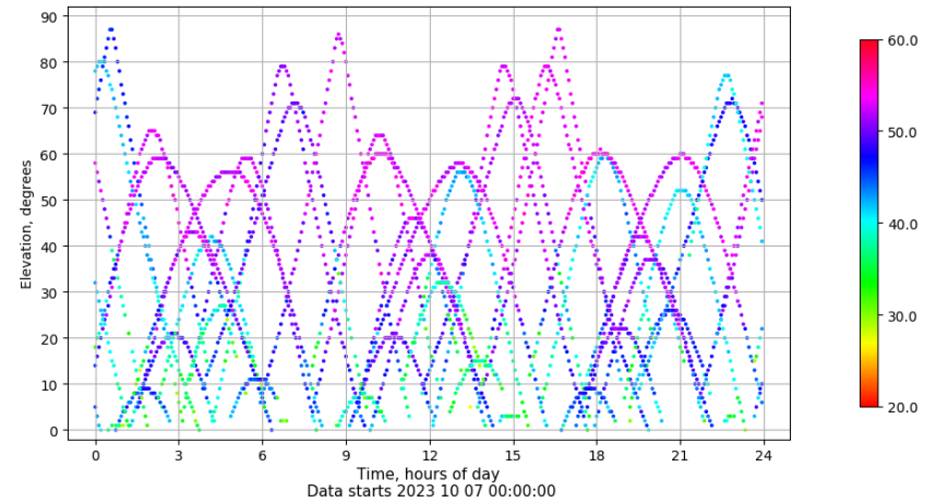
Time-elevation plot for station EIVI. Signal to Noise S1C Data file EIVI00ESP_R_2023280.xtr
