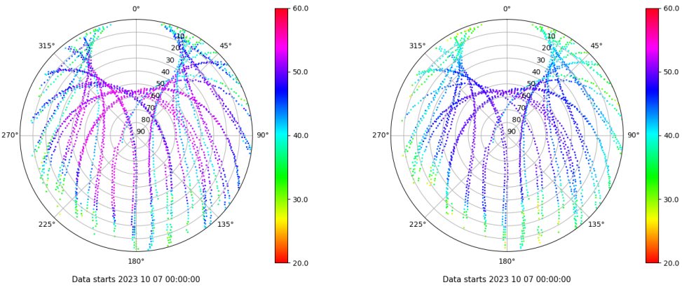
Skyplot for station EIVI. Signal to Noise S1C Data file EIVI00ESP_R_2023280.xtr Skyplot for station EIVI. Signal to Noise S2P Data file EIVI00ESP_R_2023280.xtr
