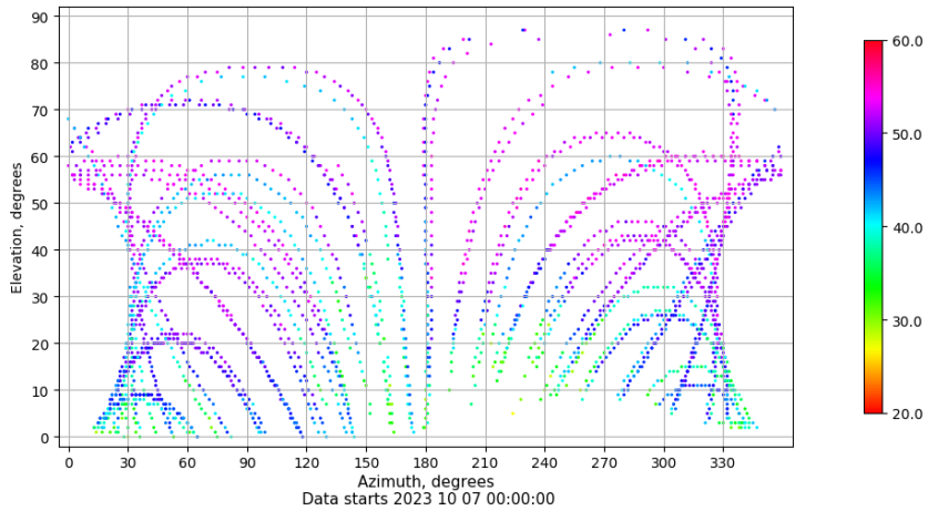
Azimuth-elevation plot for station EIVI. Signal to Noise S1C Data file EIVI00ESP_R_2023280.xtr
