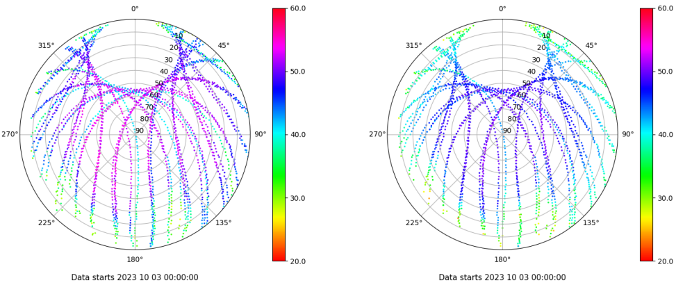
Skyplot for station EIVI. Signal to Noise S1C Data file EIVI00ESP_R_2023276.xtr Skyplot for station EIVI. Signal to Noise S2P Data file EIVI00ESP_R_2023276.xtr
