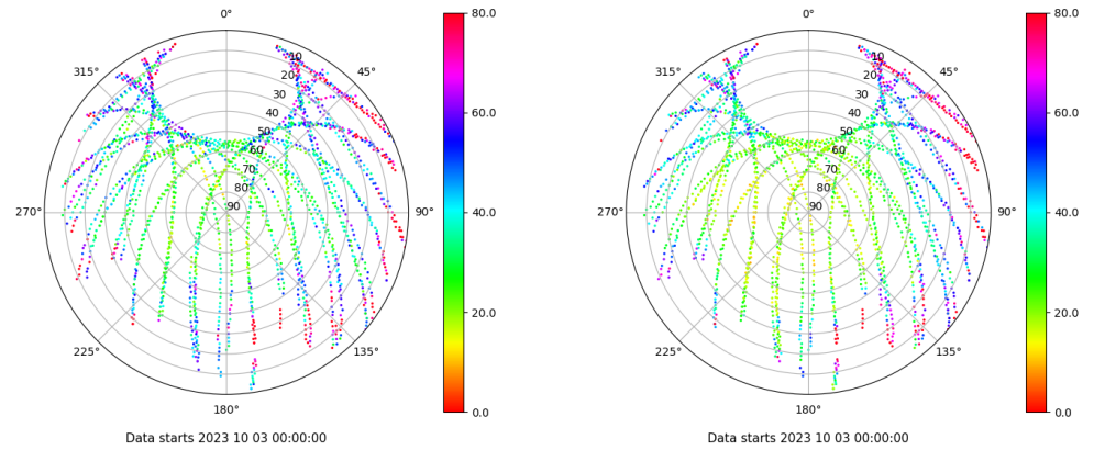
Skyplot for station EIVI. Parameter M1C Data file EIVI00ESP_R_2023276.xtr Skyplot for station EIVI. Parameter M2P Data file EIVI00ESP_R_2023276.xtr
