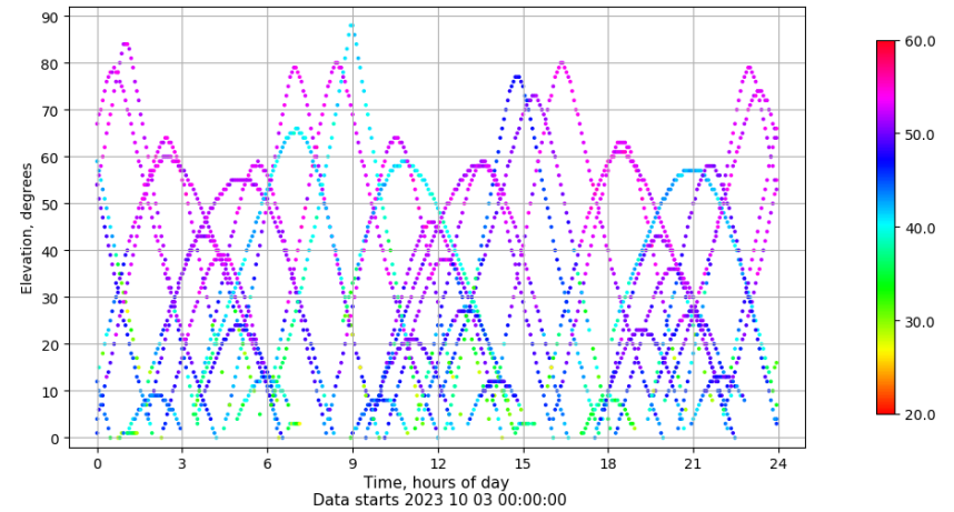
Time-elevation plot for station EIVI. Signal to Noise S1C Data file EIVI00ESP_R_2023276.xtr
