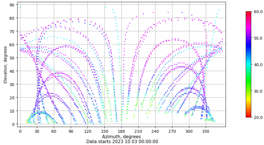
Azimuth-elevation plot for station EIVI. Signal to Noise S1C Data file EIVI00ESP_R_2023276.xtr
