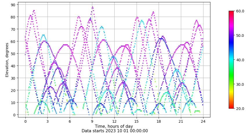
Time-elevation plot for station EIVI. Signal to Noise S1C Data file EIVI00ESP_R_2023274.xtr
