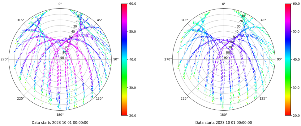
Skyplot for station EIVI. Signal to Noise S1C Data file EIVI00ESP_R_2023274.xtr Skyplot for station EIVI. Signal to Noise S2P Data file EIVI00ESP_R_2023274.xtr
