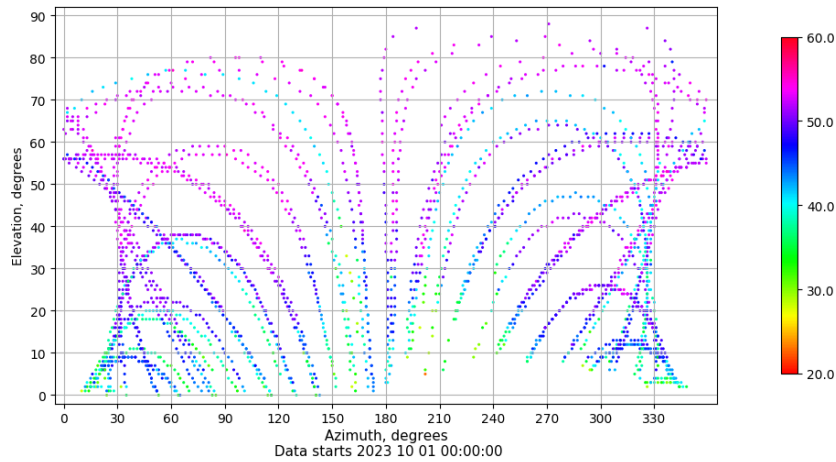
Azimuth-elevation plot for station EIVI. Signal to Noise S1C Data file EIVI00ESP_R_2023274.xtr
