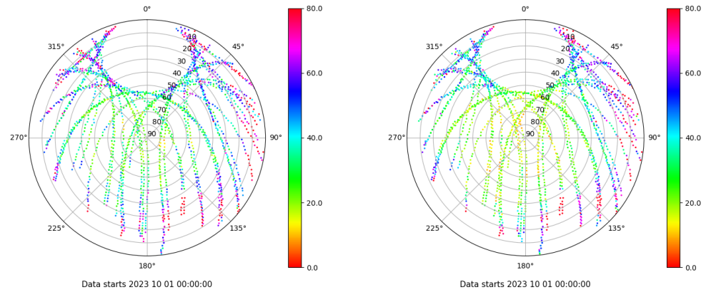
Skyplot for station EIVI. Parameter M1C Data file EIVI00ESP_R_2023274.xtr Skyplot for station EIVI. Parameter M2P Data file EIVI00ESP_R_2023274.xtr
