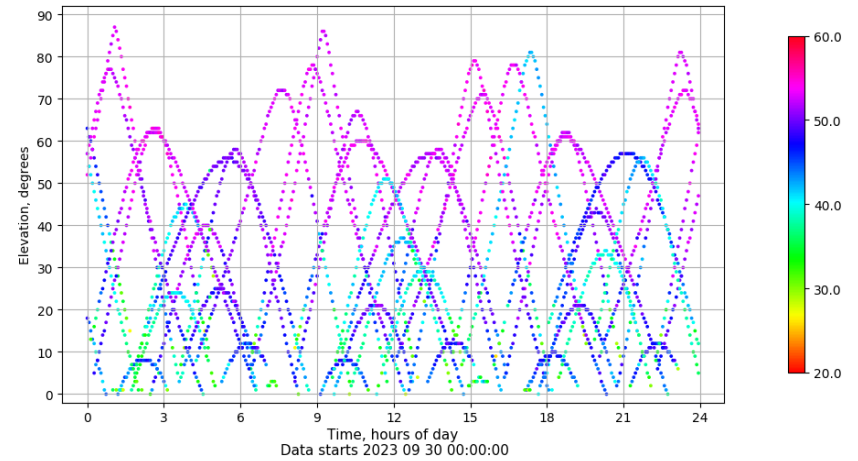
Time-elevation plot for station EIVI. Signal to Noise S1C Data file EIVI00ESP_R_2023273.xtr
