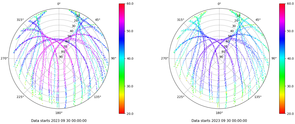
Skyplot for station EIVI. Signal to Noise S1C Data file EIVI00ESP_R_2023273.xtr Skyplot for station EIVI. Signal to Noise S2P Data file EIVI00ESP_R_2023273.xtr
