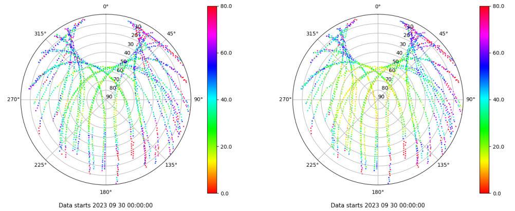
Skyplot for station EIVI. Parameter M1C Data file EIVI00ESP_R_2023273.xtr Skyplot for station EIVI. Parameter M2P Data file EIVI00ESP_R_2023273.xtr
