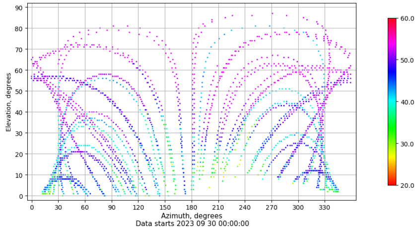
Azimuth-elevation plot for station EIVI. Signal to Noise S1C Data file EIVI00ESP_R_2023273.xtr
