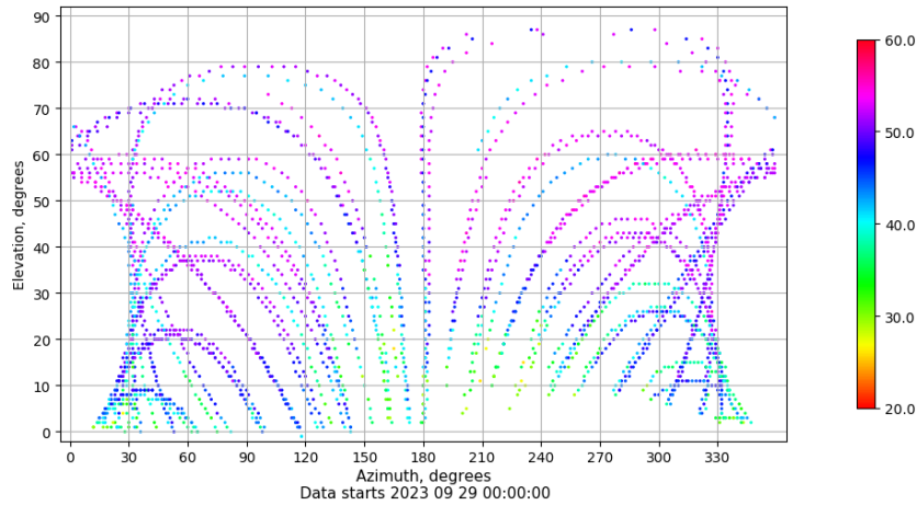
Azimuth-elevation plot for station EIVI. Signal to Noise S1C Data file EIVI00ESP_R_2023272.xtr
