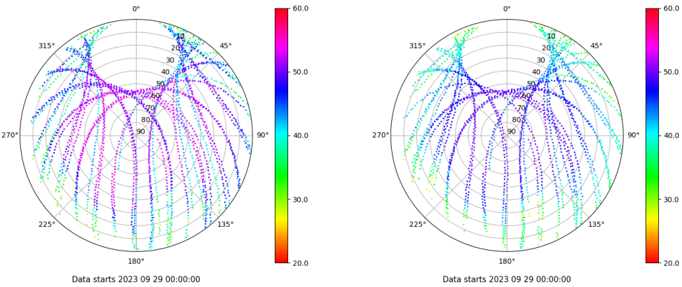
Skyplot for station EIVI. Signal to Noise S1C Data file EIVI00ESP_R_2023272.xtr Skyplot for station EIVI. Signal to Noise S2P Data file EIVI00ESP_R_2023272.xtr
