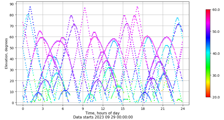
Time-elevation plot for station EIVI. Signal to Noise S1C Data file EIVI00ESP_R_2023272.xtr
