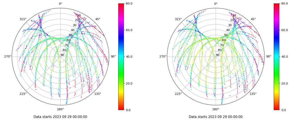
Skyplot for station EIVI. Parameter M1C Data file EIVI00ESP_R_2023272.xtr Skyplot for station EIVI. Parameter M2P Data file EIVI00ESP_R_2023272.xtr
