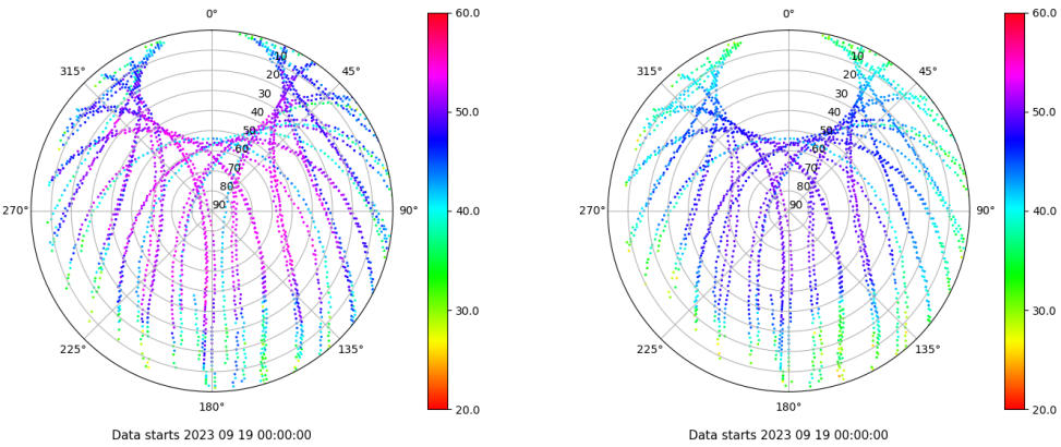
Skyplot for station EIVI. Signal to Noise S1C Data file EIVI00ESP_R_2023262.xtr Skyplot for station EIVI. Signal to Noise S2P Data file EIVI00ESP_R_2023262.xtr
