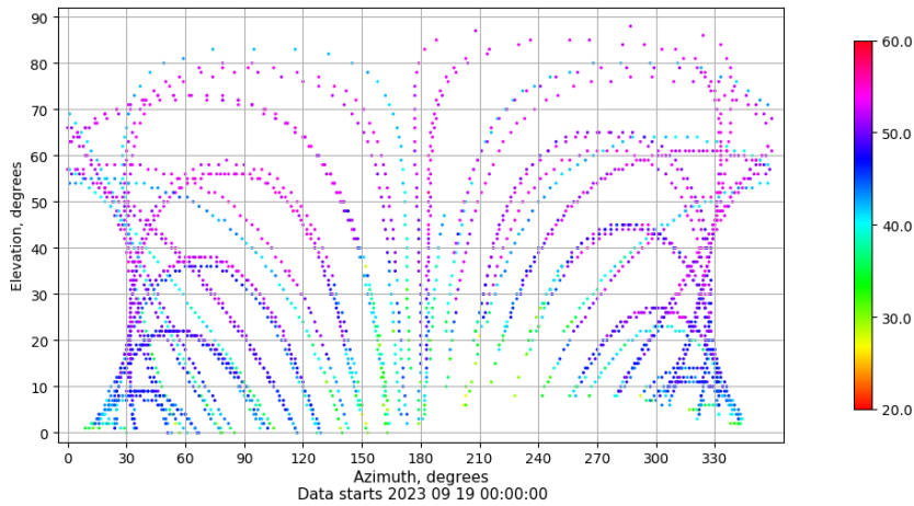
Azimuth-elevation plot for station EIVI. Signal to Noise S1C Data file EIVI00ESP_R_2023262.xtr
