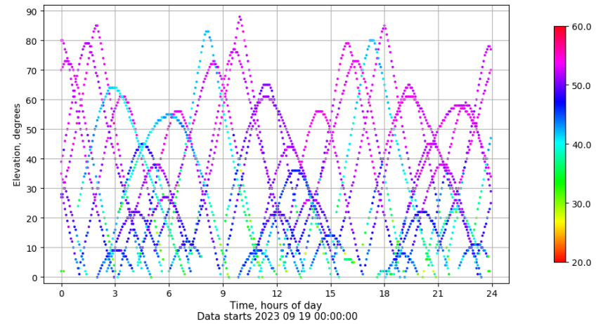
Time-elevation plot for station EIVI. Signal to Noise S1C Data file EIVI00ESP_R_2023262.xtr
