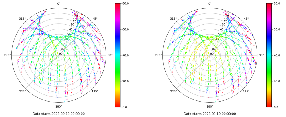
Skyplot for station EIVI. Parameter M1C Data file EIVI00ESP_R_2023262.xtr Skyplot for station EIVI. Parameter M2P Data file EIVI00ESP_R_2023262.xtr
