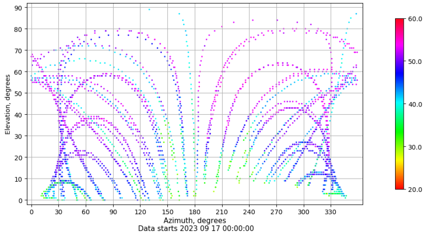
Azimuth-elevation plot for station EIVI. Signal to Noise S1C Data file EIVI00ESP_R_2023260.xtr
