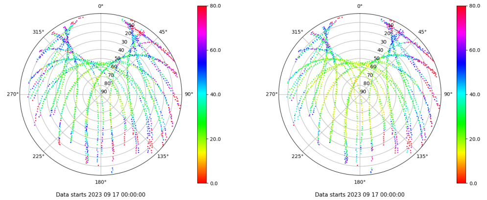
Skyplot for station EIVI. Parameter M1C Data file EIVI00ESP_R_2023260.xtr Skyplot for station EIVI. Parameter M2P Data file EIVI00ESP_R_2023260.xtr
