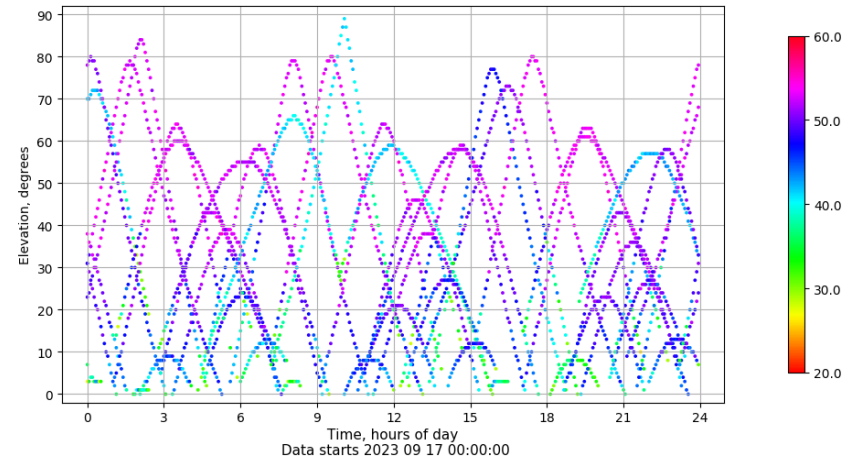
Time-elevation plot for station EIVI. Signal to Noise S1C Data file EIVI00ESP_R_2023260.xtr
