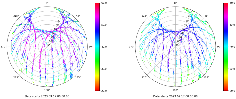
Skyplot for station EIVI. Signal to Noise S1C Data file EIVI00ESP_R_2023260.xtr Skyplot for station EIVI. Signal to Noise S2P Data file EIVI00ESP_R_2023260.xtr
