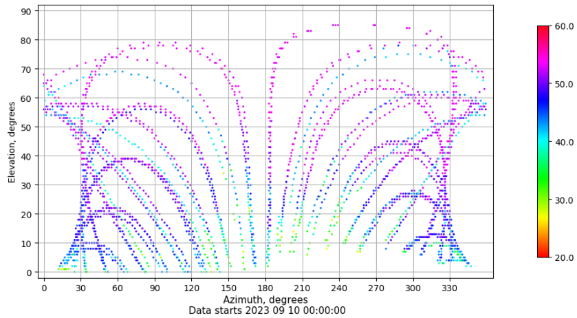
Azimuth-elevation plot for station EIVI. Signal to Noise S1C Data file EIVI00ESP_R_2023253.xtr
