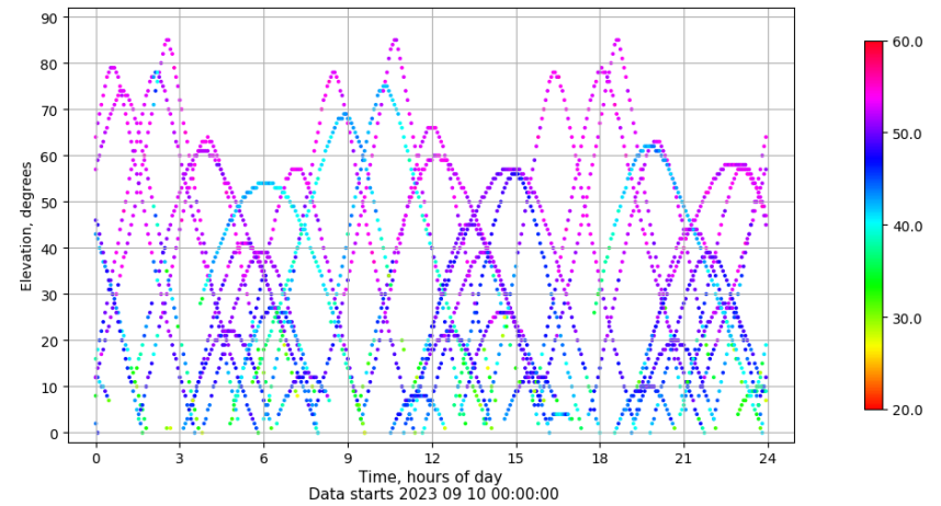
Time-elevation plot for station EIVI. Signal to Noise S1C Data file EIVI00ESP_R_2023253.xtr
