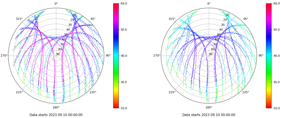
Skyplot for station EIVI. Signal to Noise S1C Data file EIVI00ESP_R_2023253.xtr Skyplot for station EIVI. Signal to Noise S2P Data file EIVI00ESP_R_2023253.xtr
