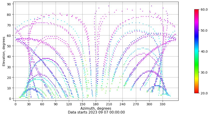
Azimuth-elevation plot for station EIVI. Signal to Noise S1C Data file EIVI00ESP_R_2023250.xtr
