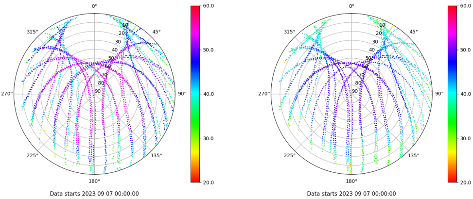
Skyplot for station EIVI. Signal to Noise S1C Data file EIVI00ESP_R_2023250.xtr Skyplot for station EIVI. Signal to Noise S2P Data file EIVI00ESP_R_2023250.xtr
