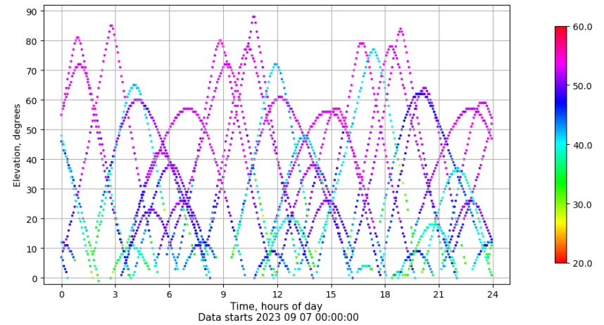
Time-elevation plot for station EIVI. Signal to Noise S1C Data file EIVI00ESP_R_2023250.xtr
