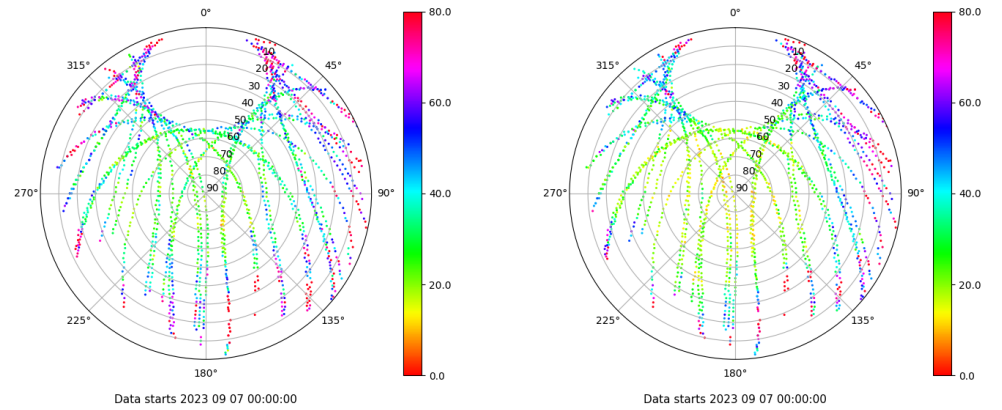
Skyplot for station EIVI. Parameter M1C Data file EIVI00ESP_R_2023250.xtr Skyplot for station EIVI. Parameter M2P Data file EIVI00ESP_R_2023250.xtr
